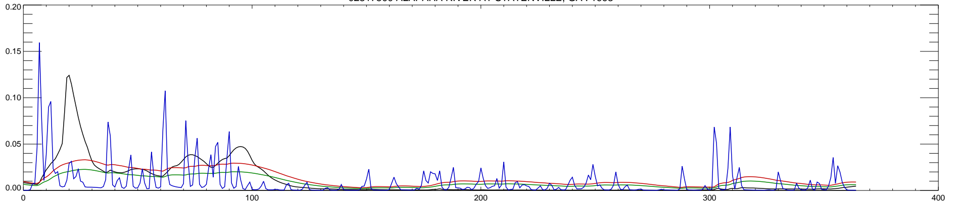
02317500 ALAPAHA RIVER AT STATENVILLE, GA : 1994
