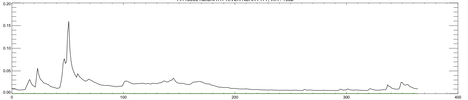
14113000 KCLICKITAT RIVER NEAR PITT, WA : 1982
