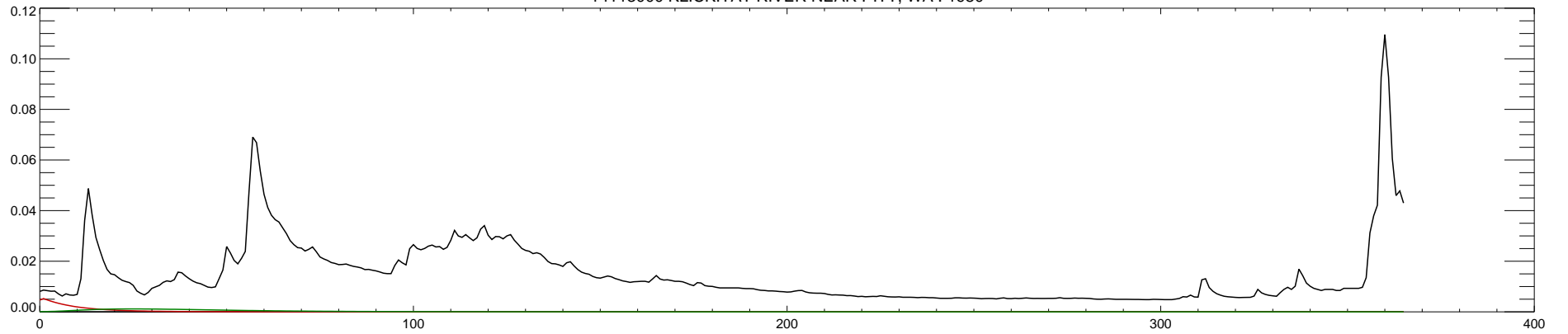
14113000 KCLICKITAT RIVER NEAR PITT, WA : 1981
