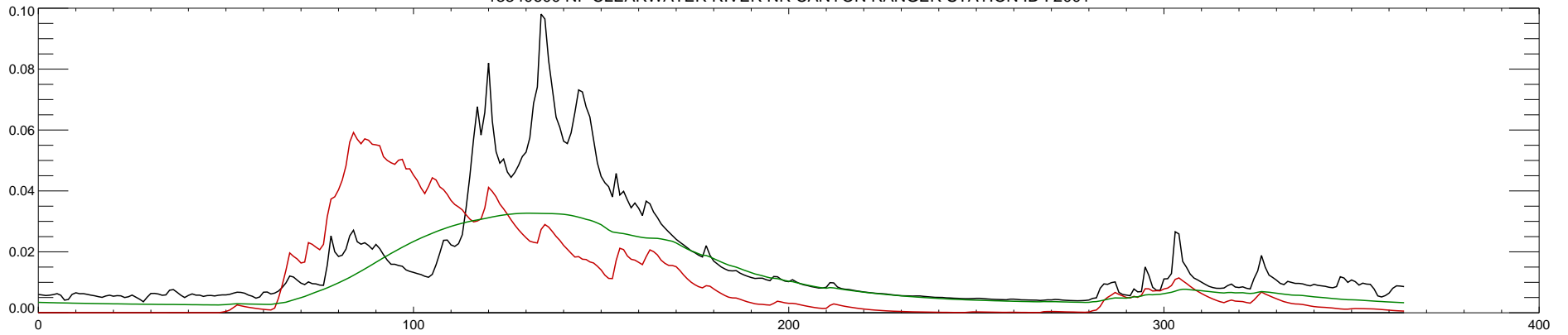
13340600 NF CLEARWATER RIVER NR CANYON RANGER STATION ID : 2002
