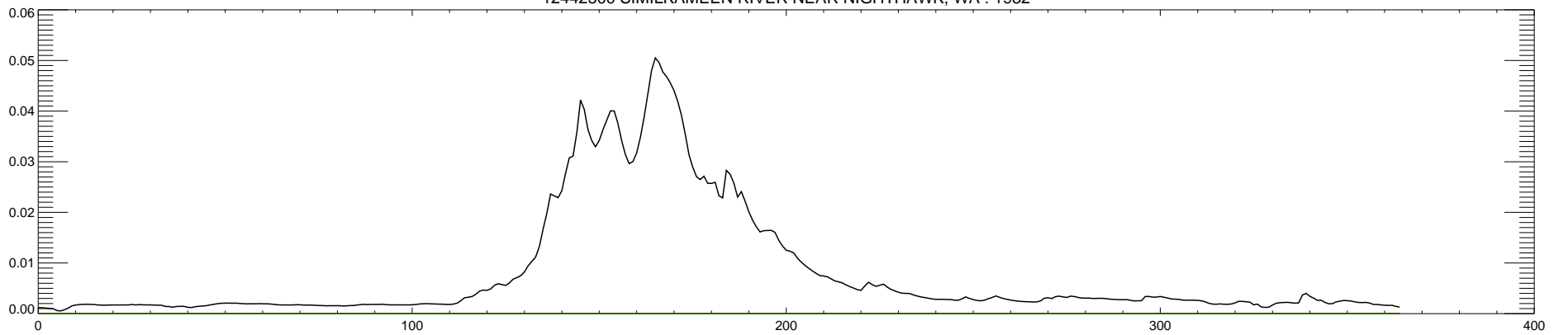
12442500 SIMILKAMEEN RIVER NEAR NIGHTHAWK, WA : 1982
