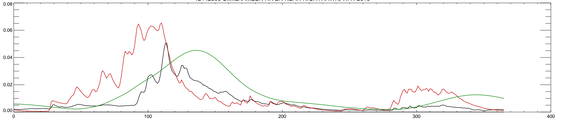
12442500 SIMILKAMEEN RIVER NEAR NIGHTHAWK, WA : 2016
