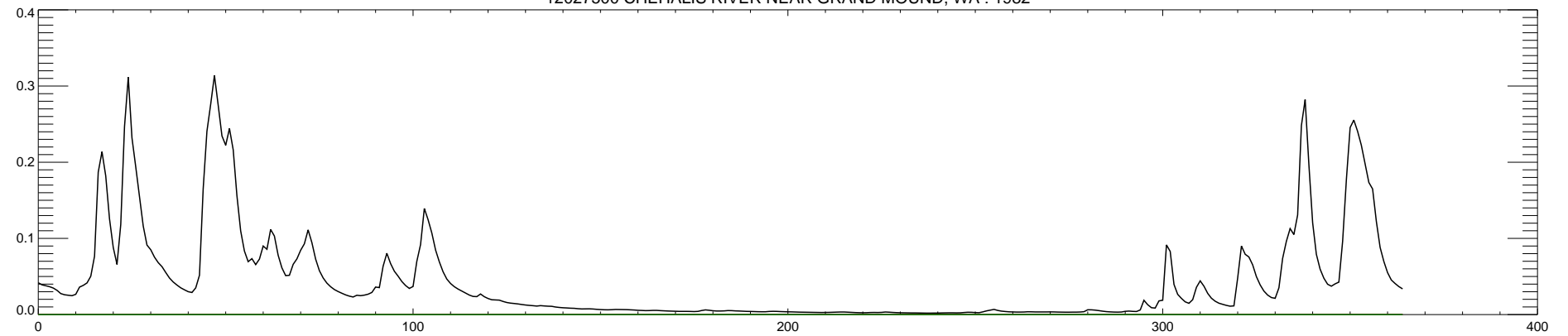
12027500 CHEHALIS RIVER NEAR GRAND MOUND, WA : 1982
