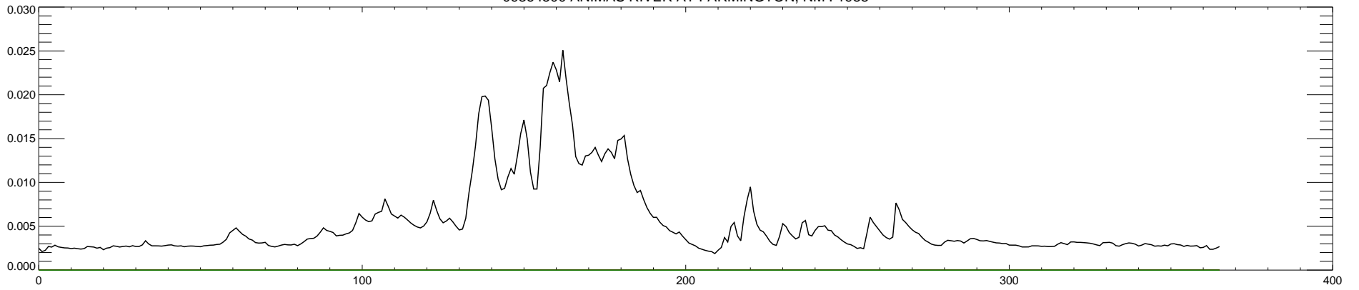
09364500 ANIMAS RIVER AT FARMINGTON, NM : 1988
