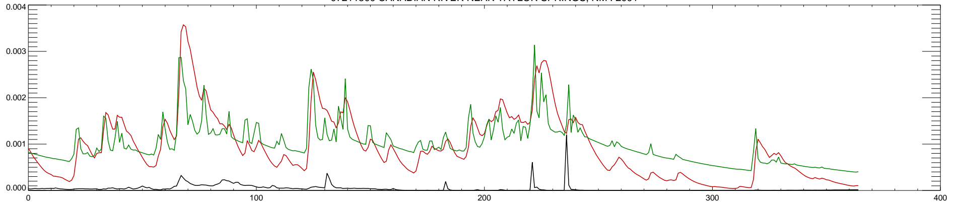
07211500 CANADIAN RIVER NEAR TAYLOR SPRINGS, NM : 2002
