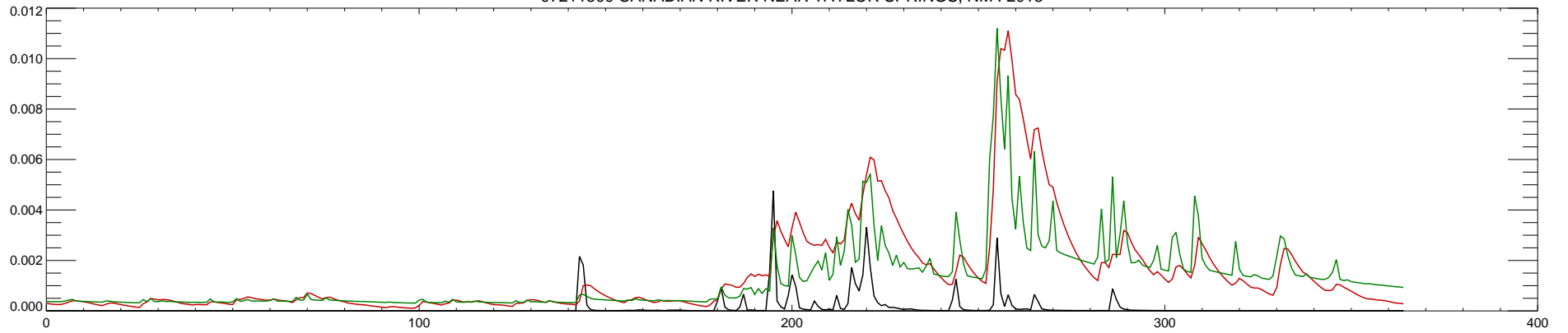
07211500 CANADIAN RIVER NEAR TAYLOR SPRINGS, NM : 2014
