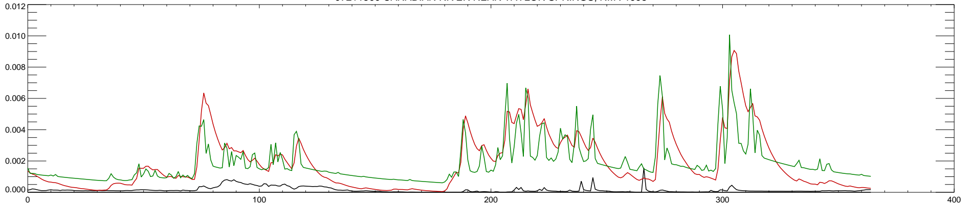
07211500 CANADIAN RIVER NEAR TAYLOR SPRINGS, NM : 1999
