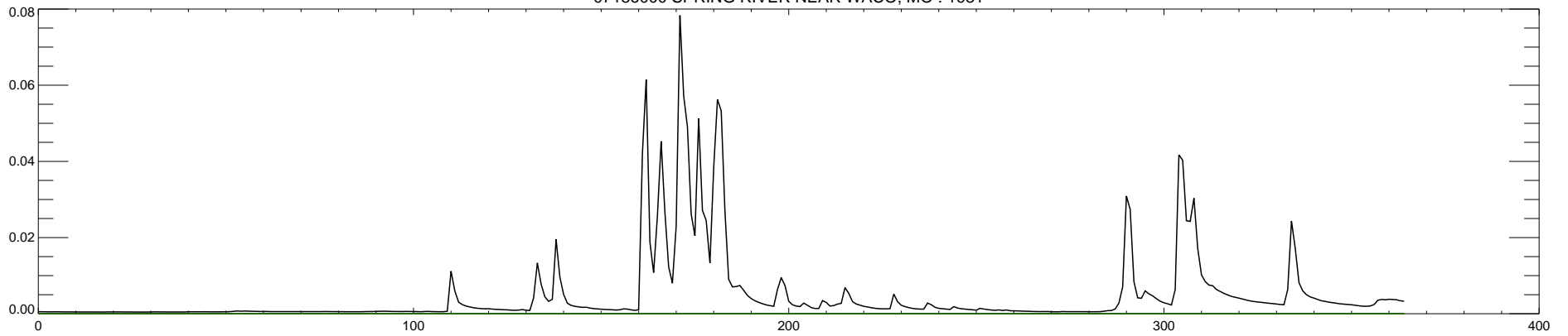
07186000 SPRING RIVER NEAR WACO, MO : 1982
