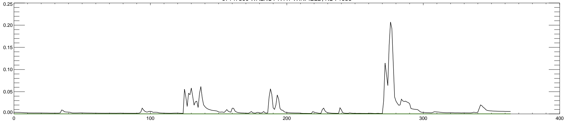
07147800 WALNUT R AT WINFIELD, KS : 1987
