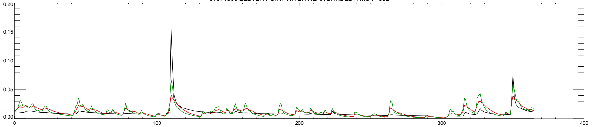
07071500 ELEVEN POINT RIVER NEAR BARDLEY, MO : 1993
