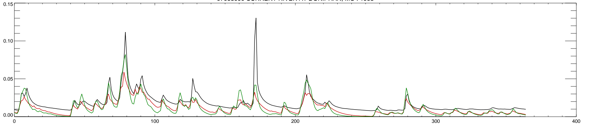
07068000 CURRENT RIVER AT DONIPHAN, MO : 1999
