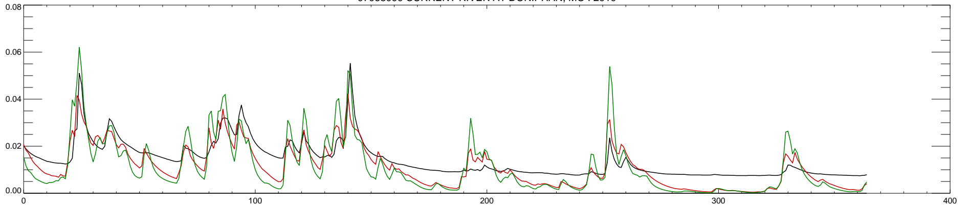
07068000 CURRENT RIVER AT DONIPHAN, MO : 2011
