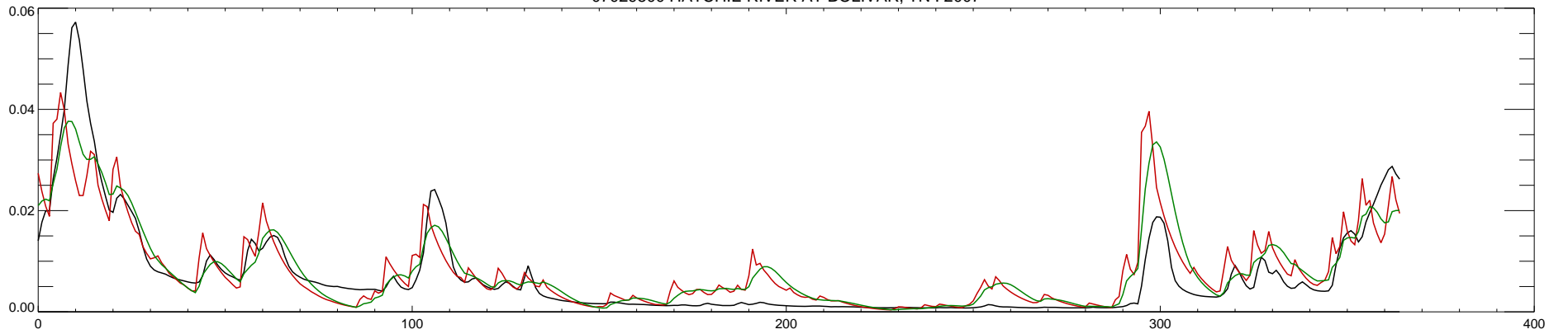
07029500 HATCHIE RIVER AT BOLIVAR, TN : 2008
