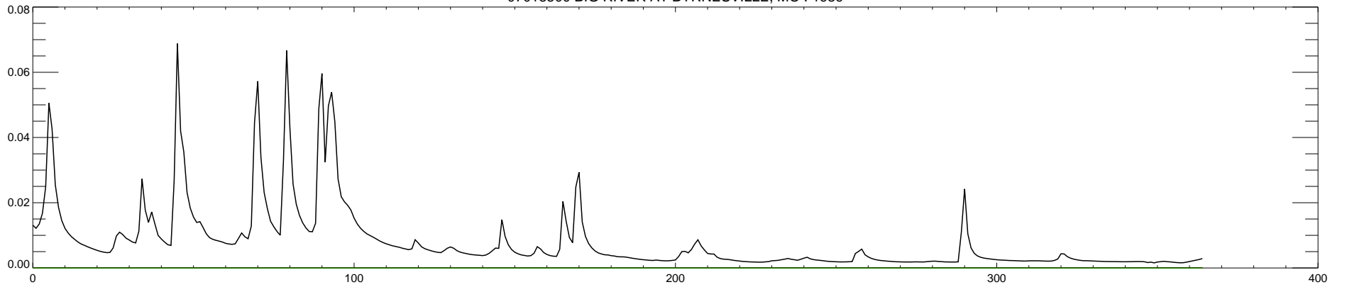
07018500 BIG RIVER AT BYRNESVILLE, MO : 1990
