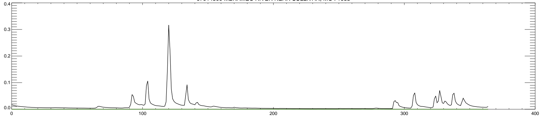
07014500 MERAMEC RIVER NEAR SULLIVAN, MO : 1984
