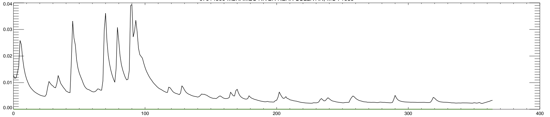
07014500 MERAMEC RIVER NEAR SULLIVAN, MO : 1990
