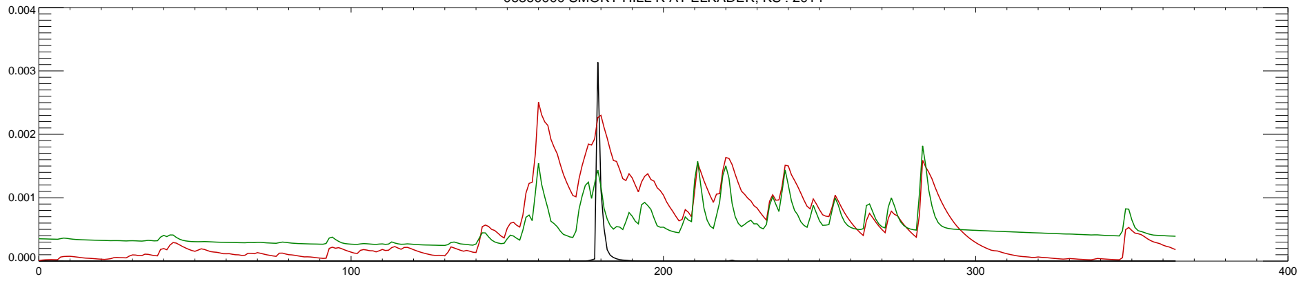
06860000 SMOKY HILL R AT ELKADER, KS : 2015
