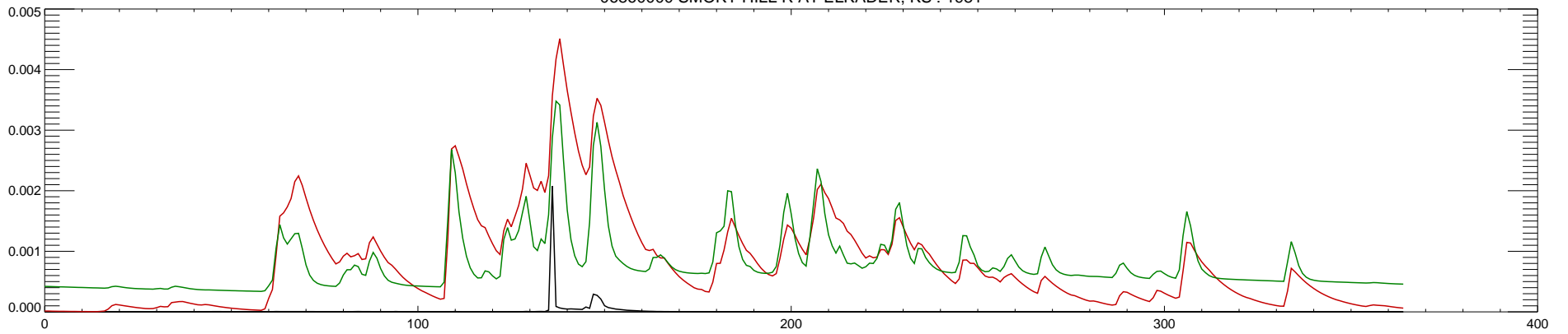
06860000 SMOKY HILL R AT ELKADER, KS : 1982
