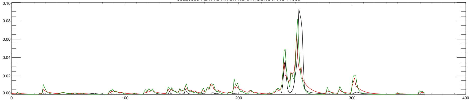
06820500 PLATTE RIVER NEAR AGENCY, MO : 1990
