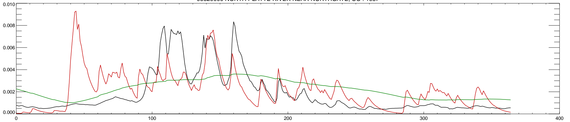
06620000 NORTH PLATTE RIVER NEAR NORTHGATE, CO : 1988
