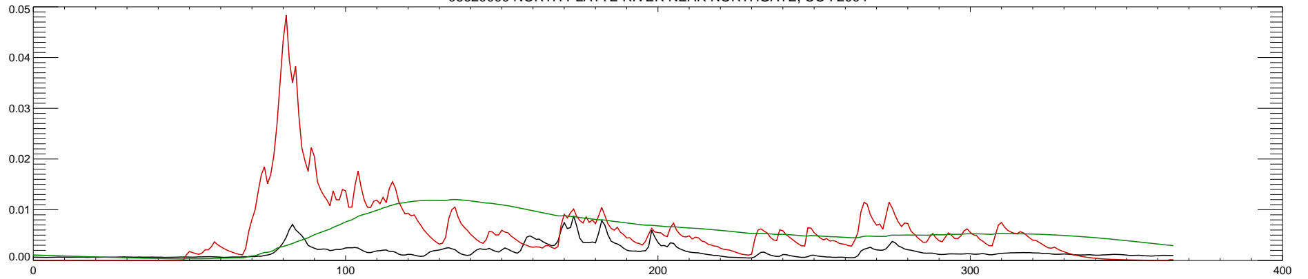
06620000 NORTH PLATTE RIVER NEAR NORTHGATE, CO : 2005
