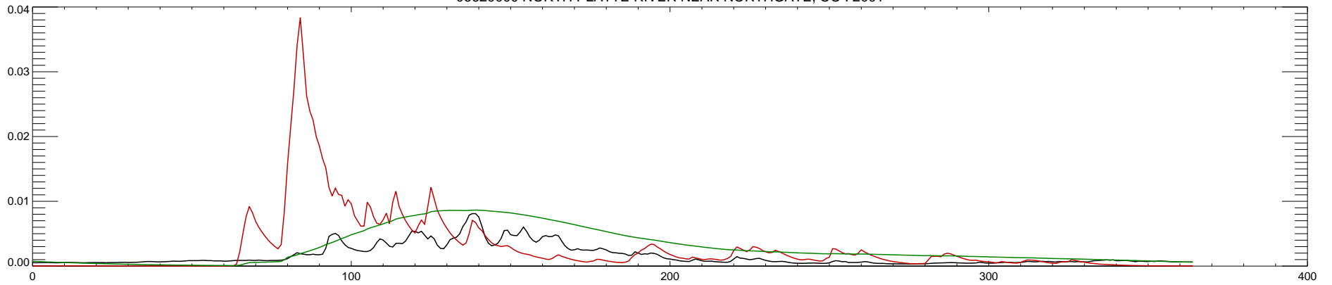
06620000 NORTH PLATTE RIVER NEAR NORTHGATE, CO : 2002
