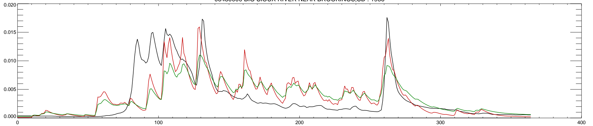
06480000 BIG SIOUX RIVER NEAR BROOKINGS,SD : 1987
