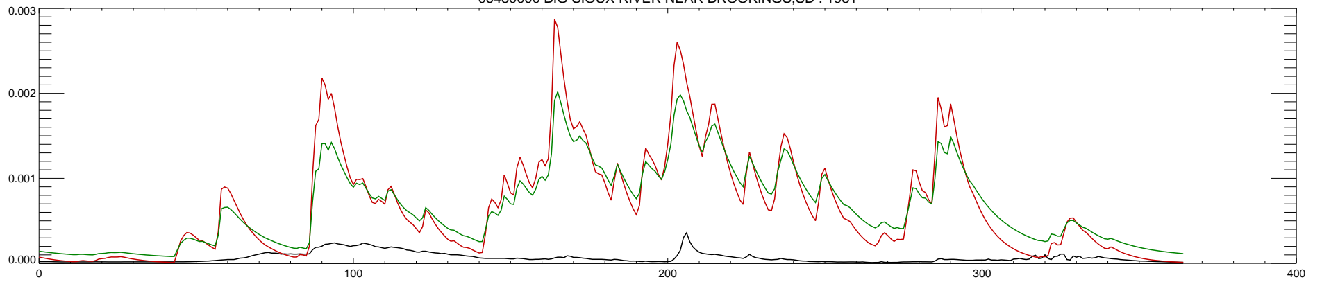
06480000 BIG SIOUX RIVER NEAR BROOKINGS,SD : 1982
