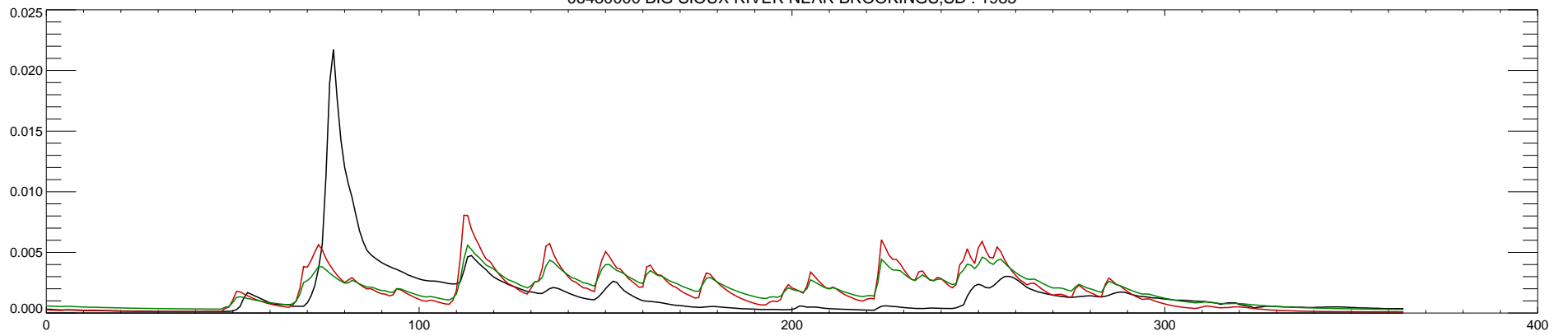
06480000 BIG SIOUX RIVER NEAR BROOKINGS,SD : 1985
