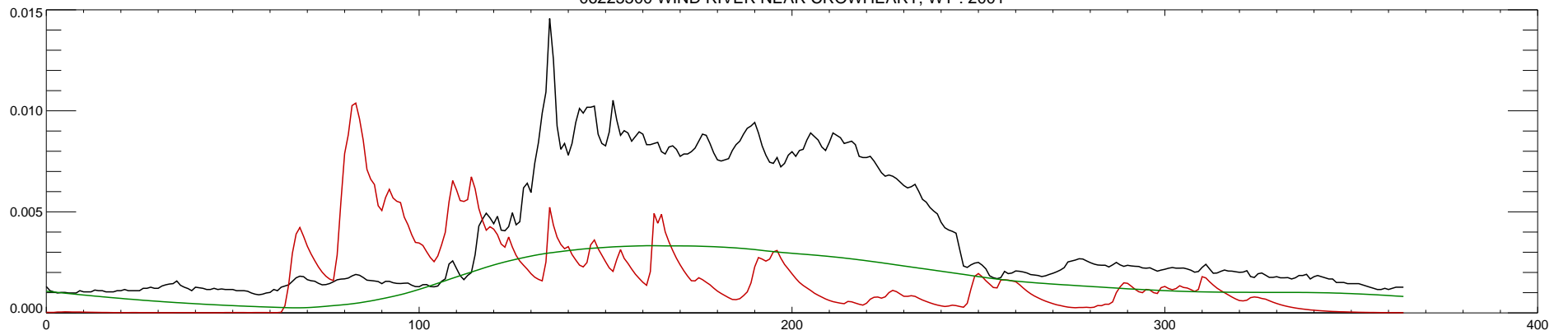
06225500 WIND RIVER NEAR CROWHEART, WY : 2002
