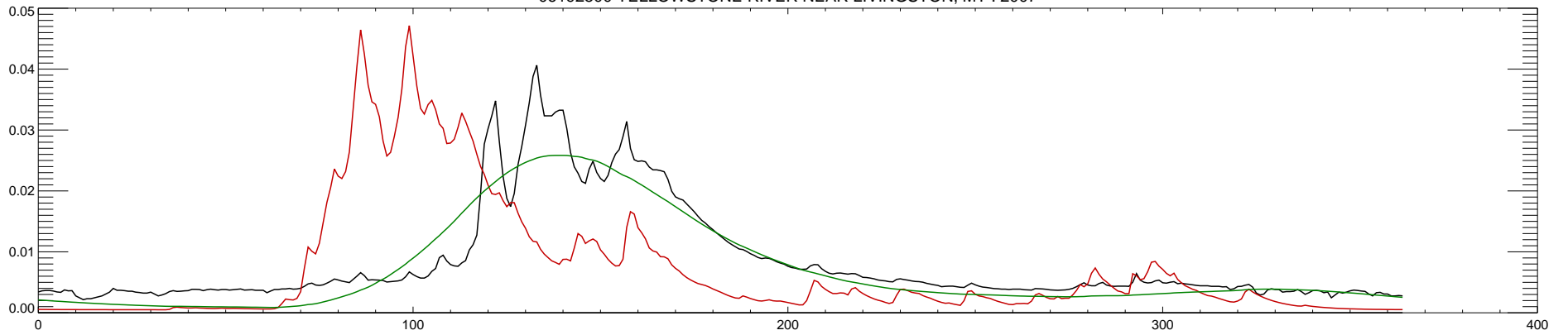
06192500 YELLOWSTONE RIVER NEAR LIVINGSTON, MT : 2008
