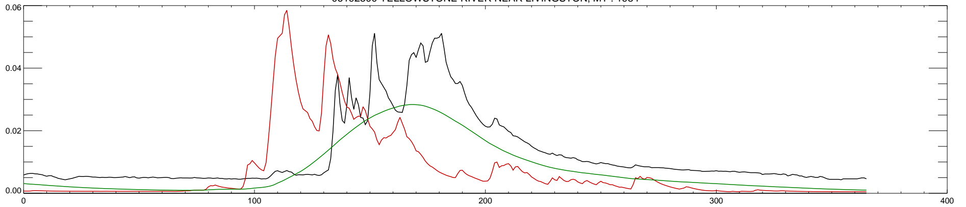
06192500 YELLOWSTONE RIVER NEAR LIVINGSTON, MT : 1985
