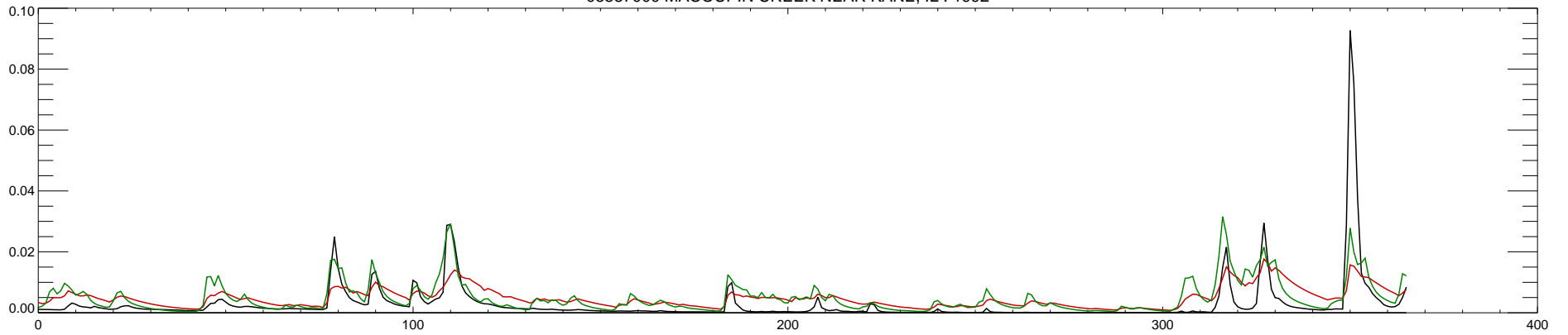
05587000 MACOUPIN CREEK NEAR KANE, IL : 1993
