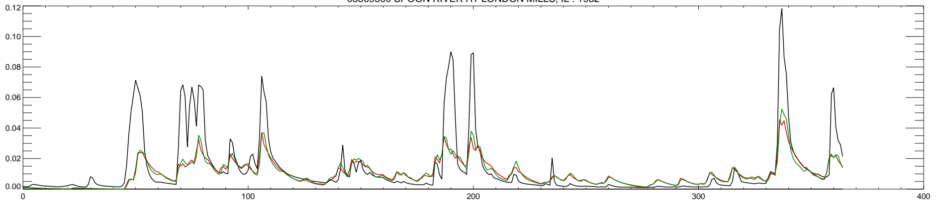
05569500 SPOON RIVER AT LONDON MILLS, IL : 1982
