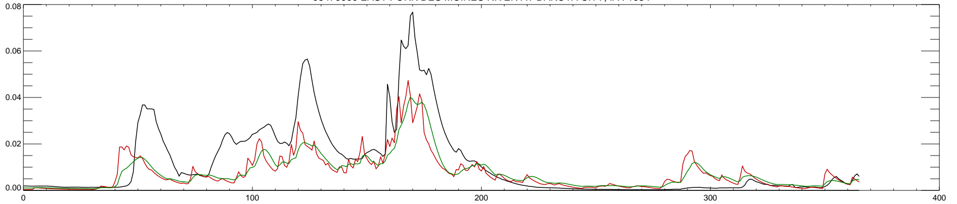
05479000 EAST FORK DES MOINES RIVER AT DAKOTA CITY, IA : 1985
