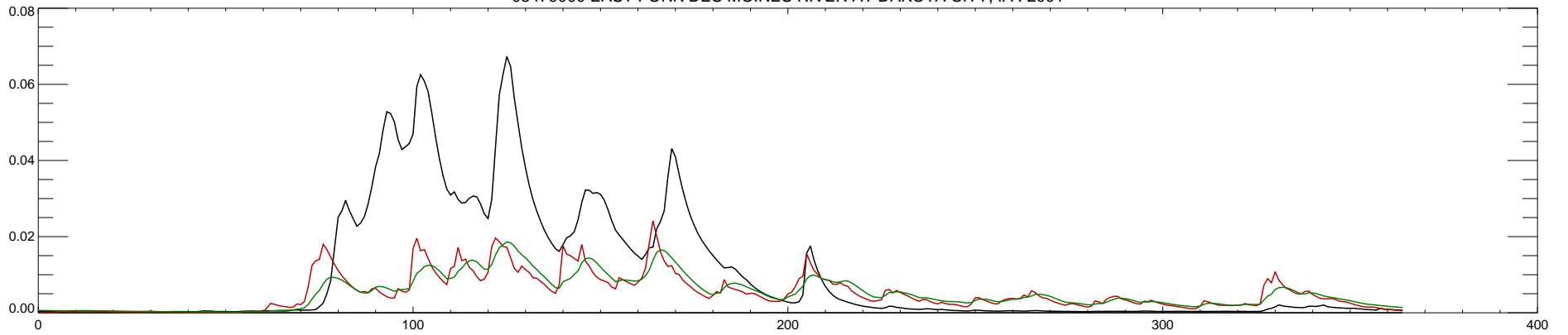
05479000 EAST FORK DES MOINES RIVER AT DAKOTA CITY, IA : 2002
