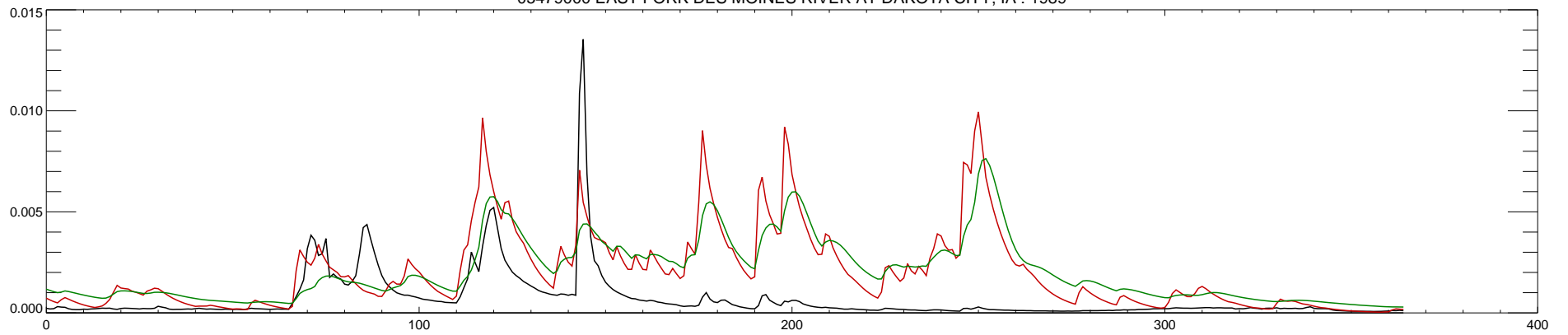
05479000 EAST FORK DES MOINES RIVER AT DAKOTA CITY, IA : 1990
