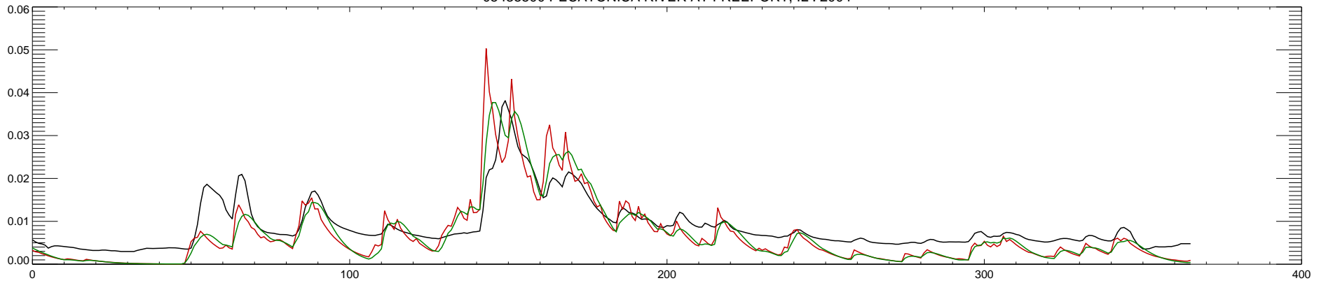
05435500 PECATONICA RIVER AT FREEPORT, IL : 2005
