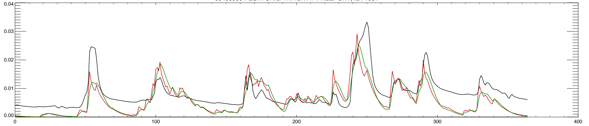
05435500 PECATONICA RIVER AT FREEPORT, IL : 1982
