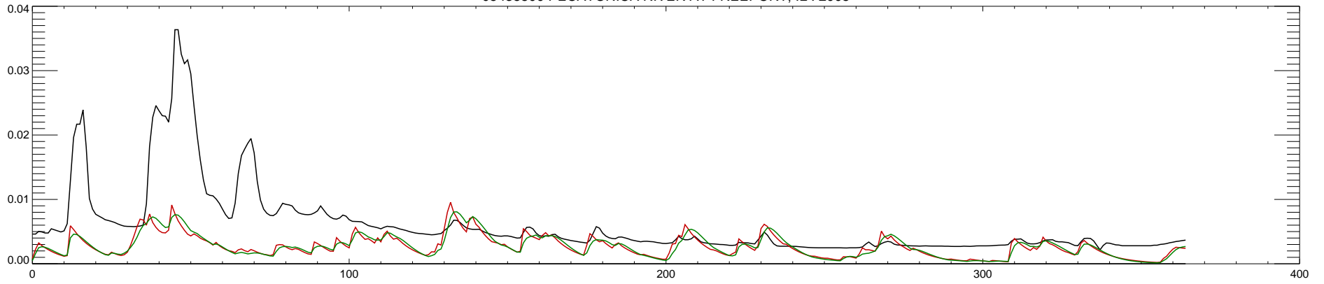
05435500 PECATONICA RIVER AT FREEPORT, IL : 2006
