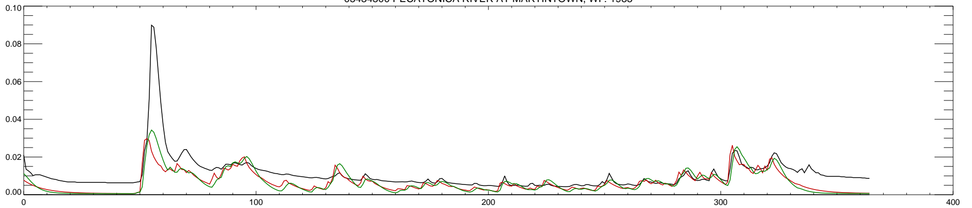
05434500 PECATONICA RIVER AT MARTINTOWN, WI : 1985
