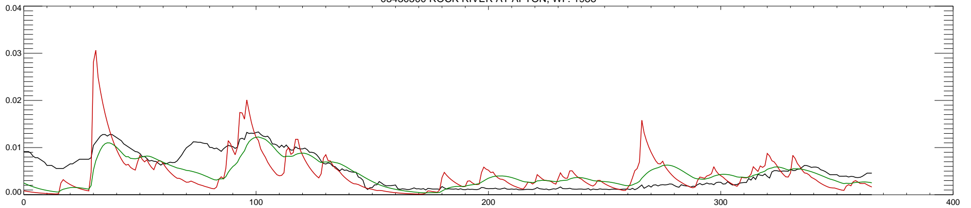
05430500 ROCK RIVER AT AFTON, WI : 1988
