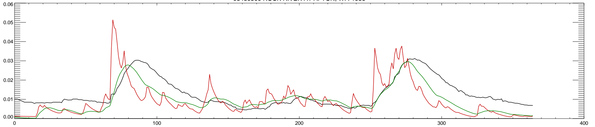
05430500 ROCK RIVER AT AFTON, WI : 1987
