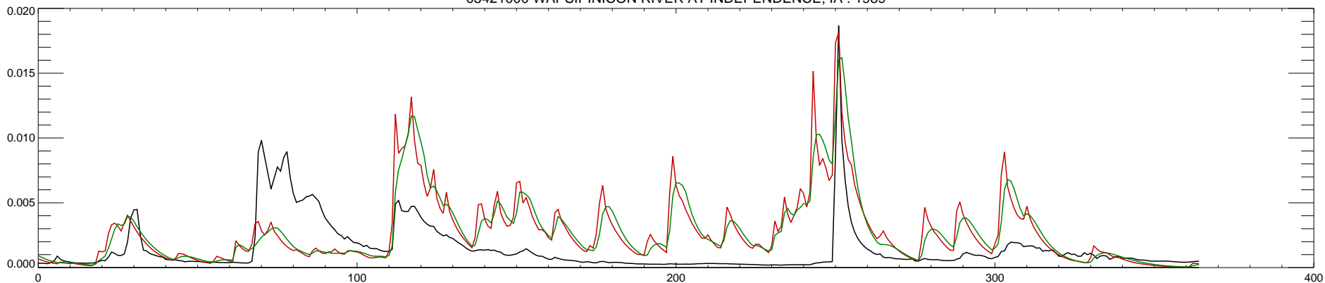
05421000 WAPSIPINICON RIVER AT INDEPENDENCE, IA : 1990
