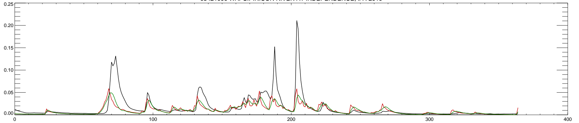
05421000 WAPSIPINICON RIVER AT INDEPENDENCE, IA : 2011
