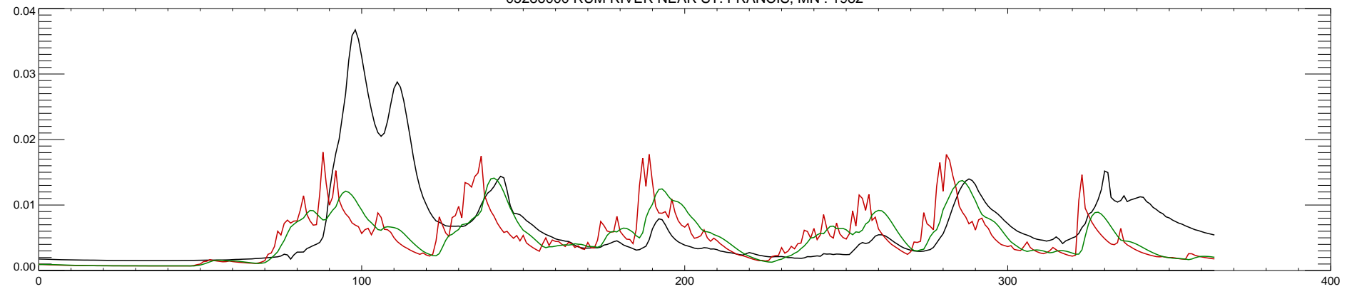
05286000 RUM RIVER NEAR ST. FRANCIS, MN : 1982
