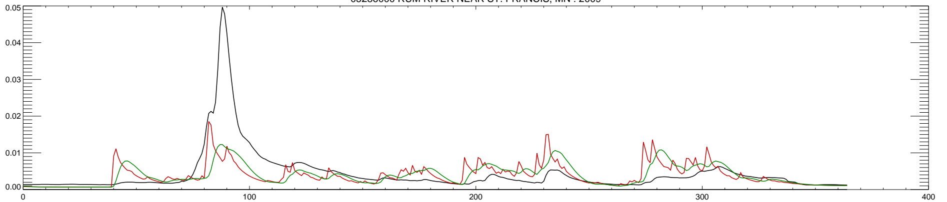
05286000 RUM RIVER NEAR ST. FRANCIS, MN : 2009
