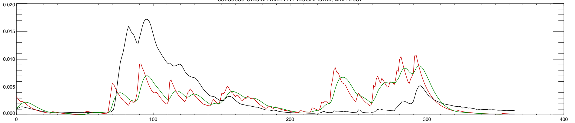
05280000 CROW RIVER AT ROCKFORD, MN : 2008
