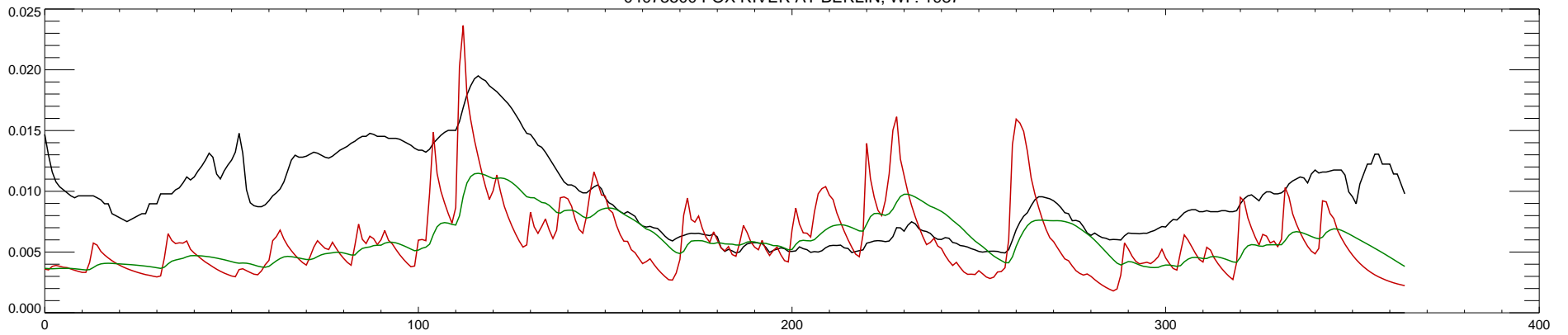
04073500 FOX RIVER AT BERLIN, WI : 1988
