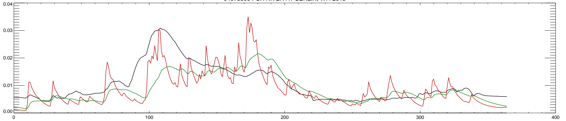
04073500 FOX RIVER AT BERLIN, WI : 2014
