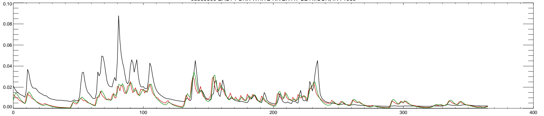
03365500 EAST FORK WHITE RIVER AT SEYMOUR, IN : 1981
