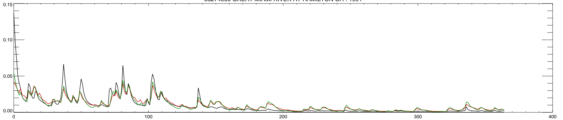
03274000 GREAT MIAMI RIVER AT HAMILTON OH : 1991
