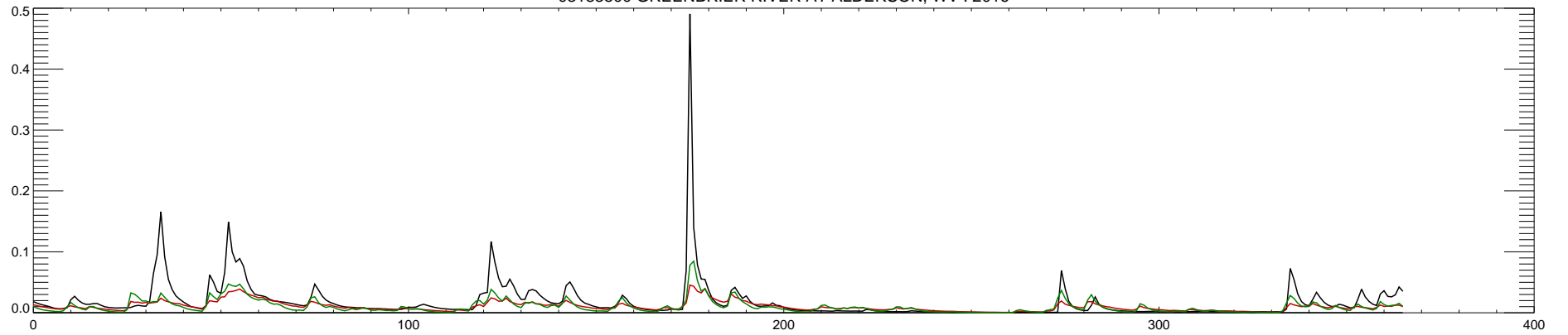
03183500 GREENBRIER RIVER AT ALDERSON, WV : 2016
