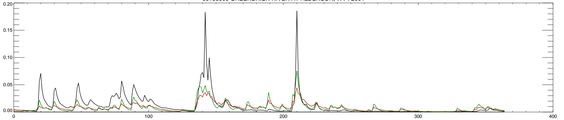
03183500 GREENBRIER RIVER AT ALDERSON, WV : 2002
