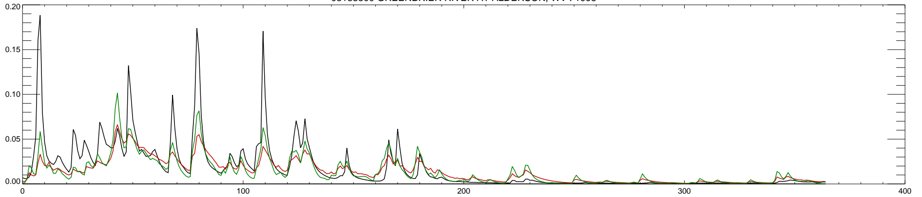
03183500 GREENBRIER RIVER AT ALDERSON, WV : 1999
