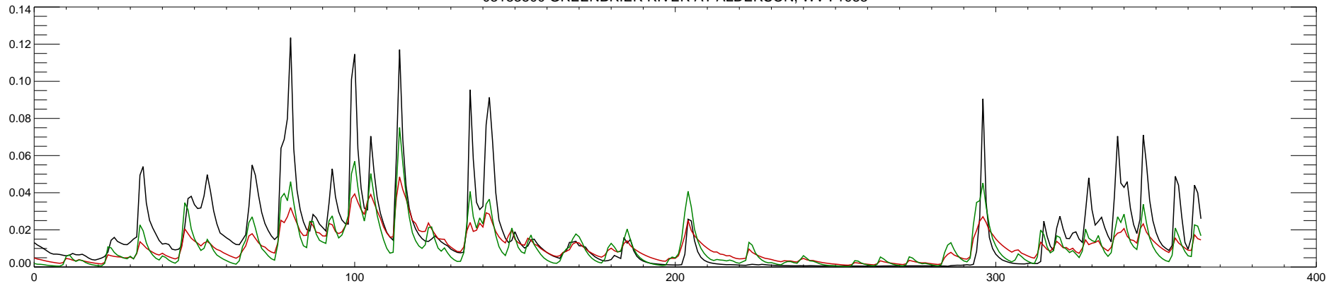
03183500 GREENBRIER RIVER AT ALDERSON, WV : 1984
