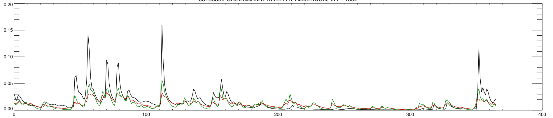
03183500 GREENBRIER RIVER AT ALDERSON, WV : 1993
