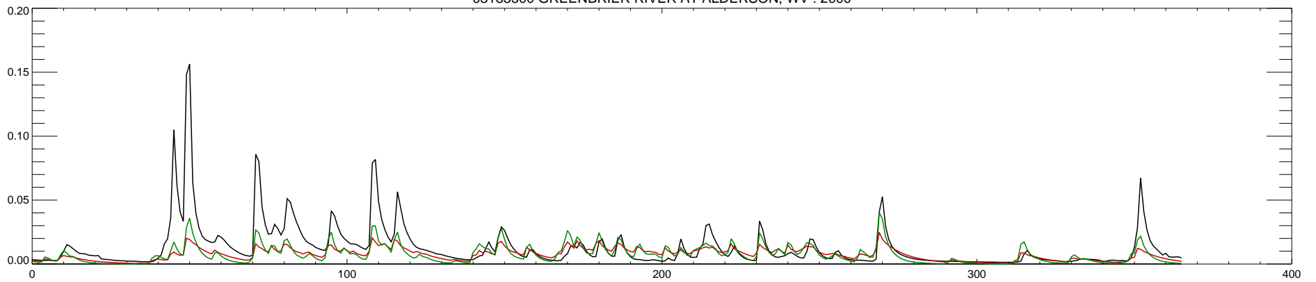
03183500 GREENBRIER RIVER AT ALDERSON, WV : 2000
