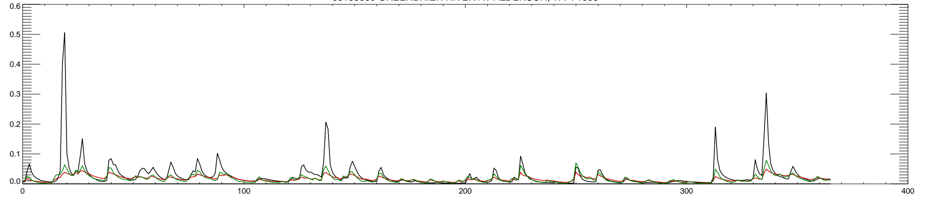
03183500 GREENBRIER RIVER AT ALDERSON, WV : 1997
