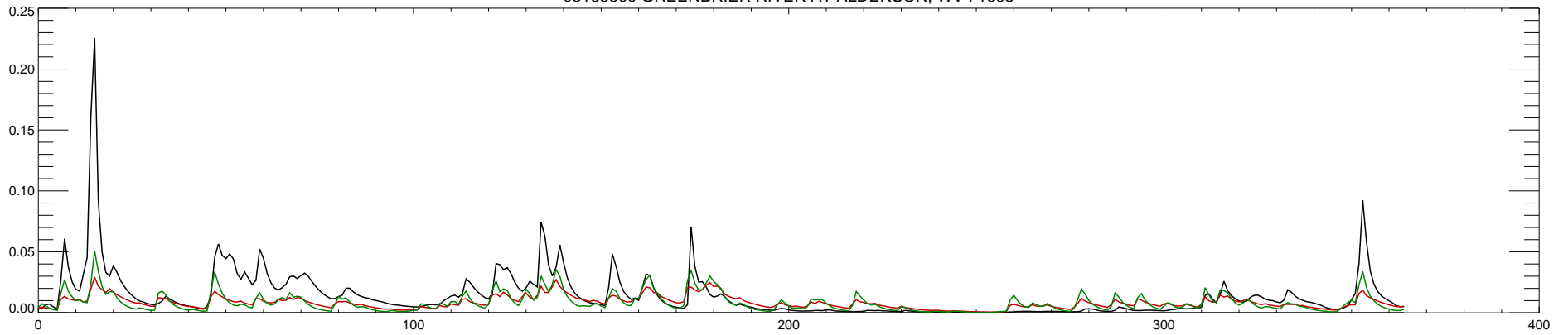
03183500 GREENBRIER RIVER AT ALDERSON, WV : 1996
