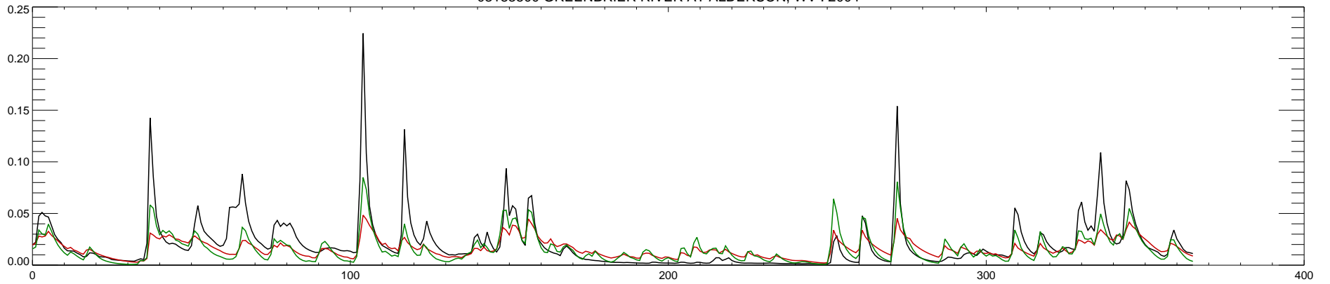
03183500 GREENBRIER RIVER AT ALDERSON, WV : 2005
