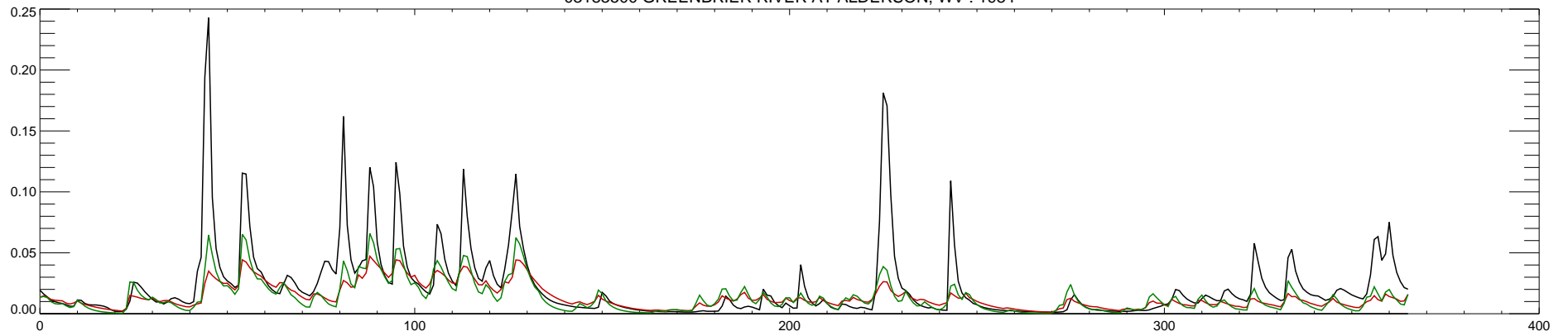
03183500 GREENBRIER RIVER AT ALDERSON, WV : 1985
