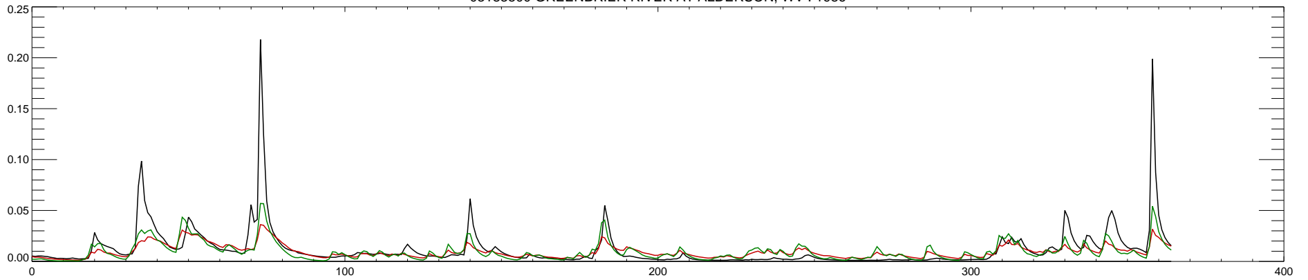
03183500 GREENBRIER RIVER AT ALDERSON, WV : 1987
