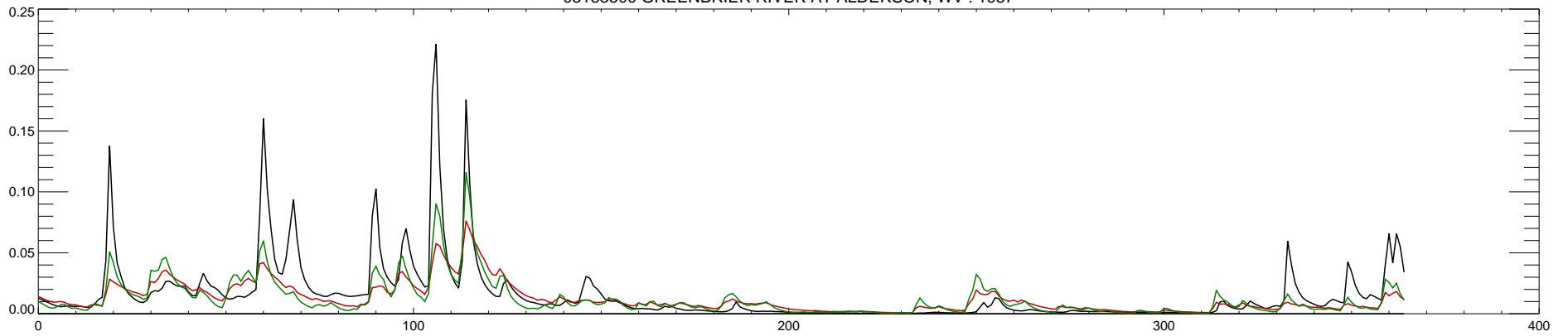
03183500 GREENBRIER RIVER AT ALDERSON, WV : 1988
