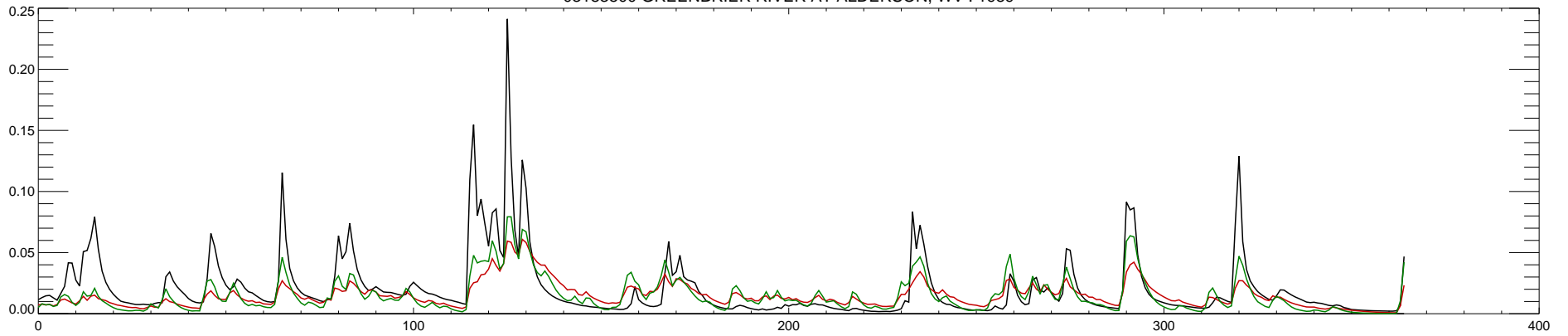
03183500 GREENBRIER RIVER AT ALDERSON, WV : 1990
