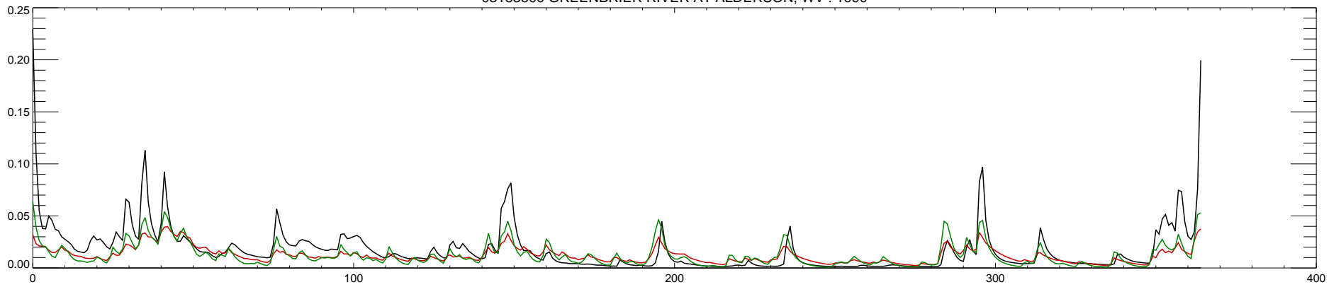
03183500 GREENBRIER RIVER AT ALDERSON, WV : 1991
