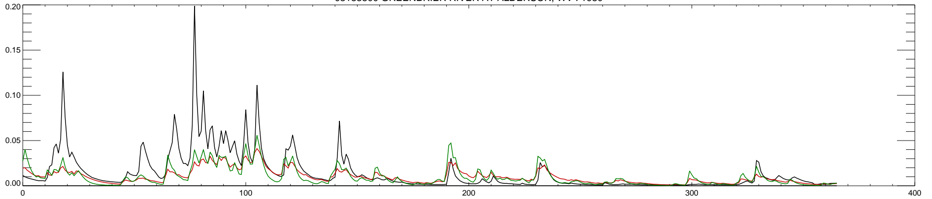
03183500 GREENBRIER RIVER AT ALDERSON, WV : 1981
