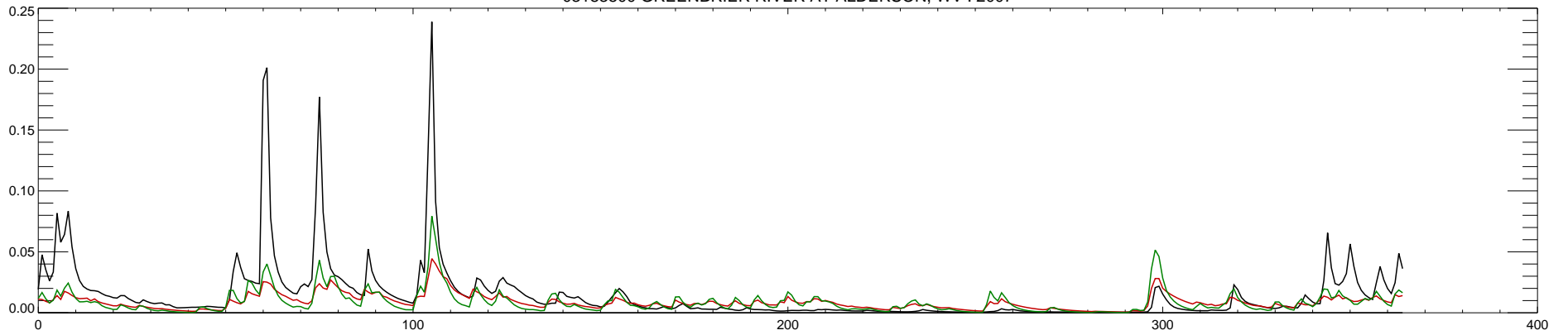
03183500 GREENBRIER RIVER AT ALDERSON, WV : 2008
