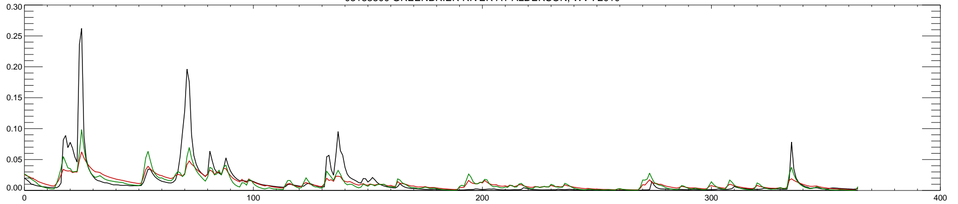
03183500 GREENBRIER RIVER AT ALDERSON, WV : 2011
