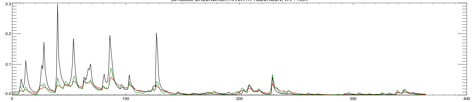
03183500 GREENBRIER RIVER AT ALDERSON, WV : 1994
