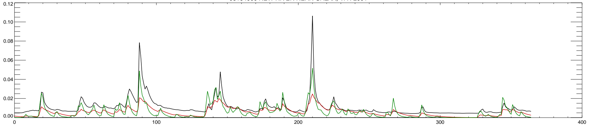
03164000 NEW RIVER NEAR GALAX, VA : 2002
