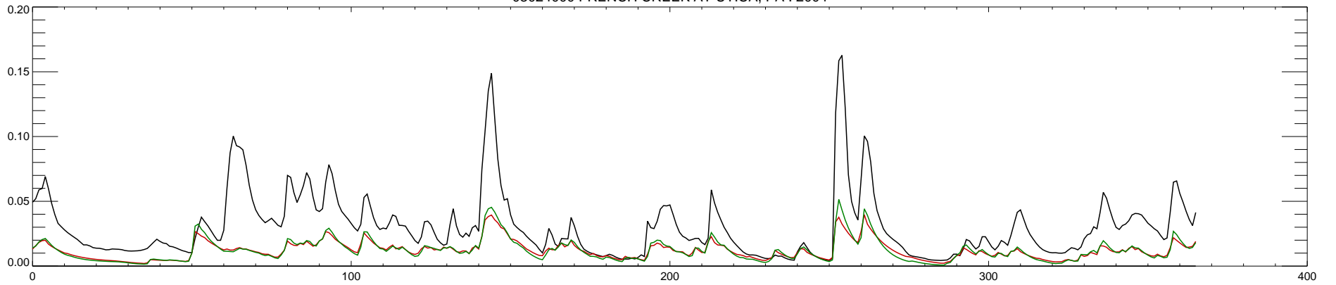
03024000 FRENCH CREEK AT UTICA, PA : 2005
