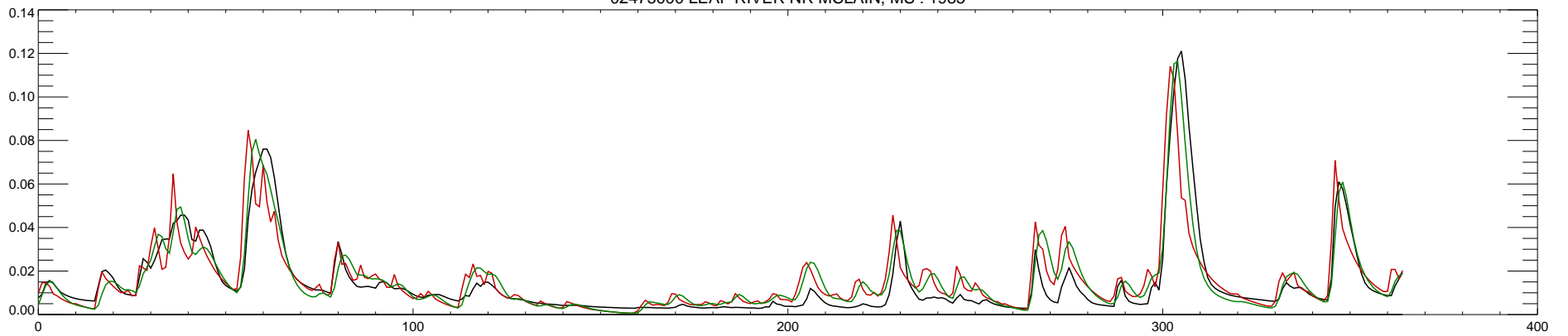
02475000 LEAF RIVER NR MCLAIN, MS : 1985
