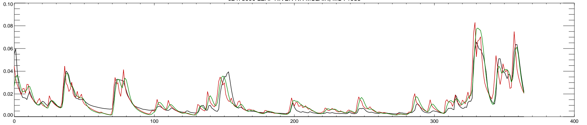
02475000 LEAF RIVER NR MCLAIN, MS : 1987
