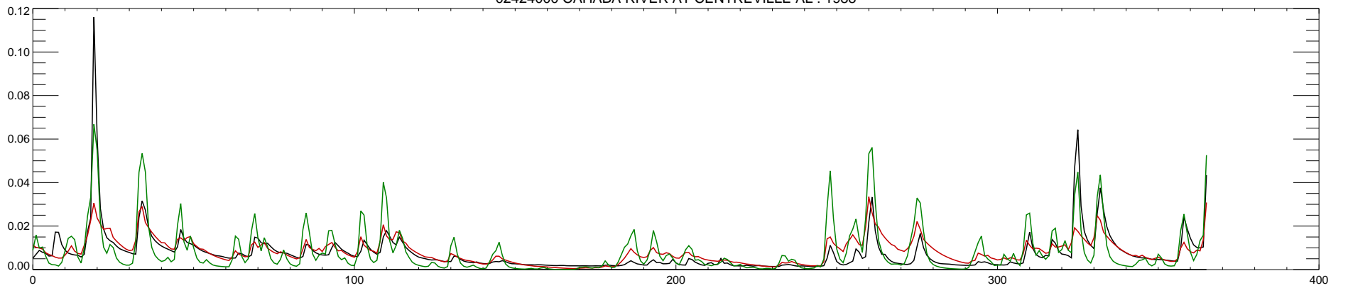
02424000 CAHABA RIVER AT CENTREVILLE AL : 1988
