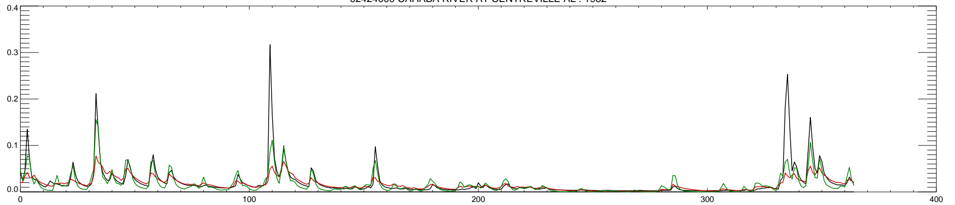
02424000 CAHABA RIVER AT CENTREVILLE AL : 1982
