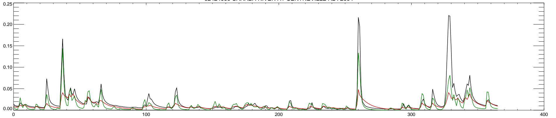
02424000 CAHABA RIVER AT CENTREVILLE AL : 2005
