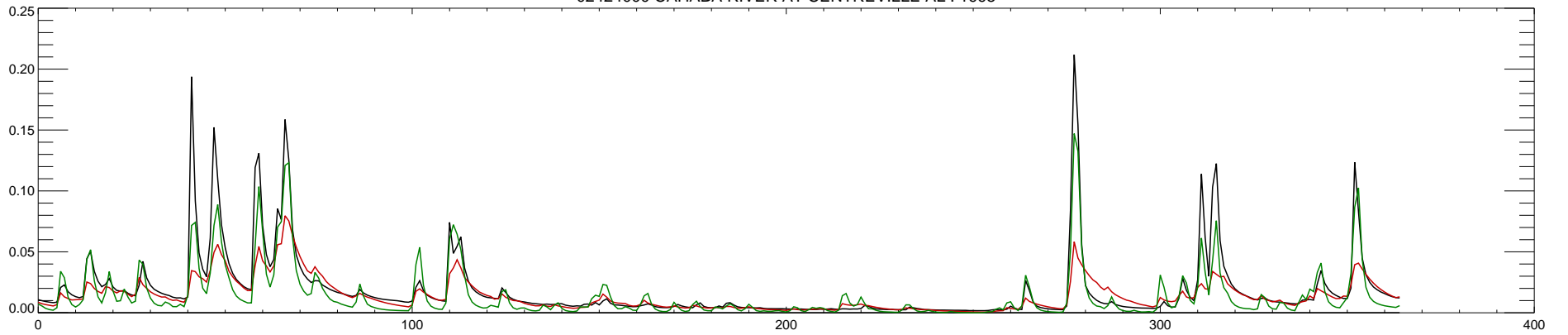
02424000 CAHABA RIVER AT CENTREVILLE AL : 1996
