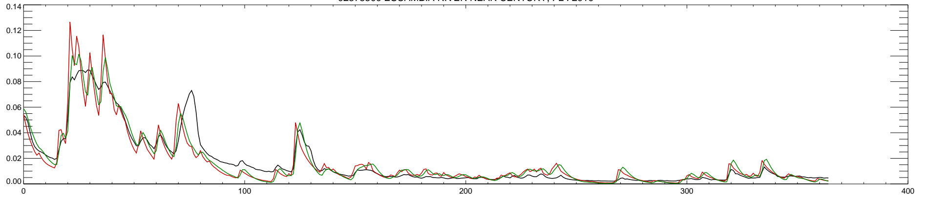
02375500 ESCAMBIA RIVER NEAR CENTURY, FL : 2011
