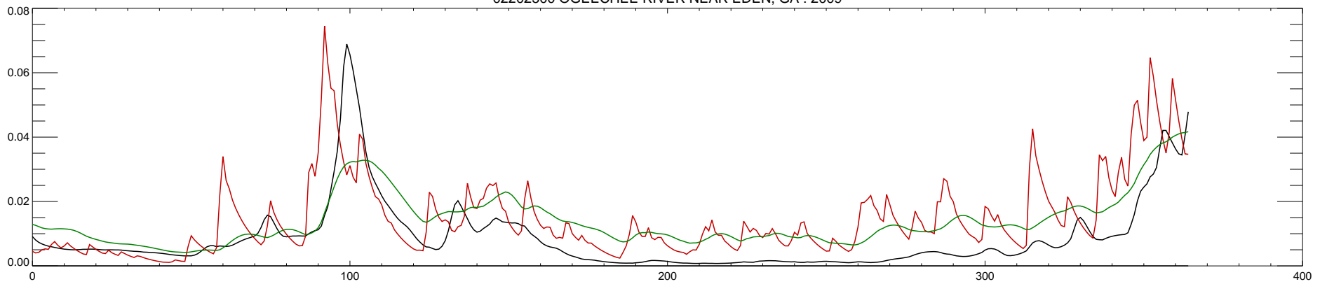
02202500 OGEECHEE RIVER NEAR EDEN, GA : 2009
