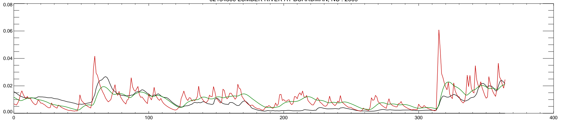
02134500 LUMBER RIVER AT BOARDMAN, NC : 2009
