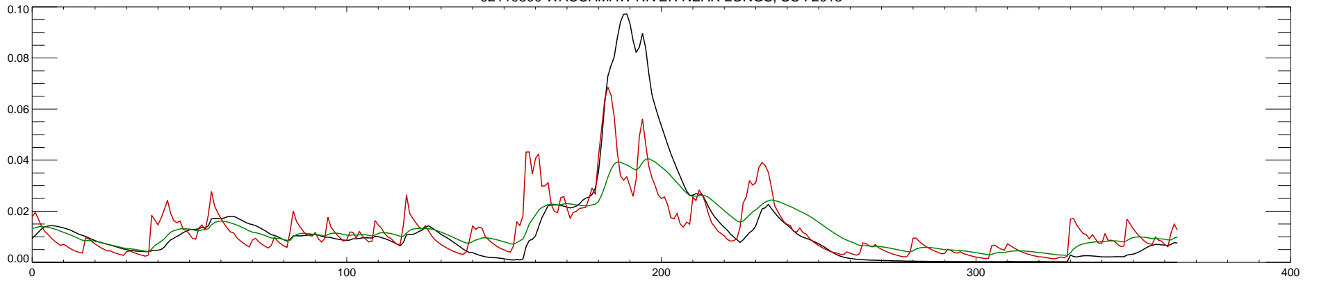
02110500 WACCAMAW RIVER NEAR LONGS, SC : 2014
