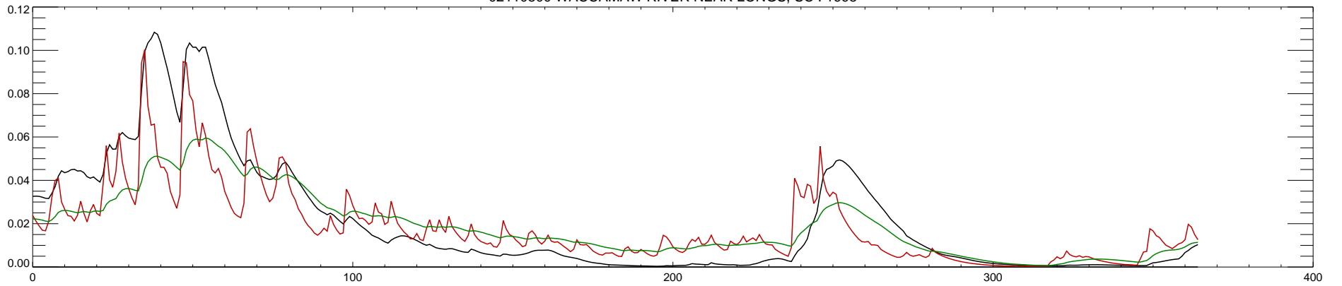
02110500 WACCAMAW RIVER NEAR LONGS, SC : 1999
