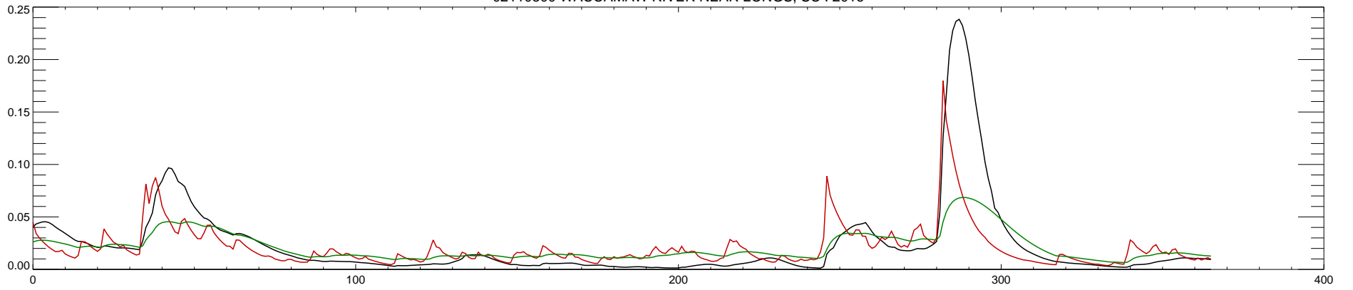
02110500 WACCAMAW RIVER NEAR LONGS, SC : 2016
