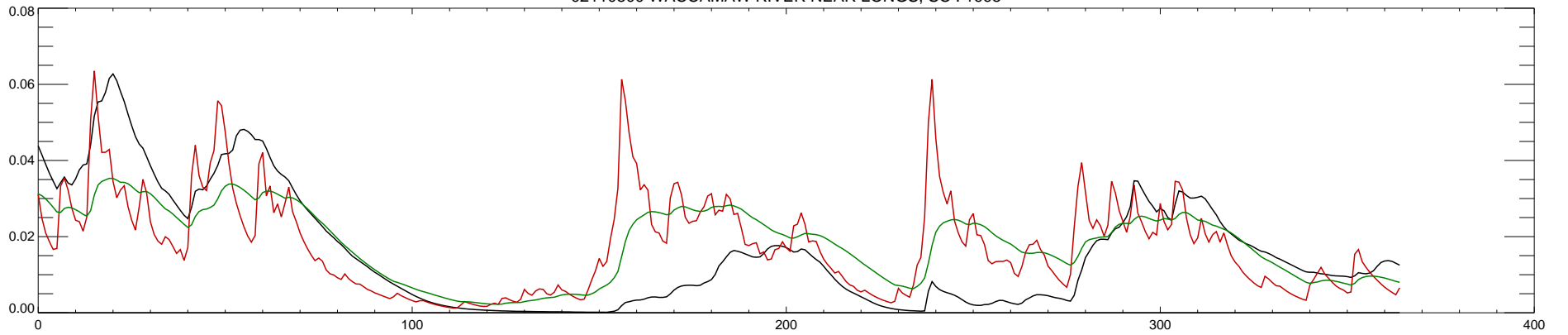
02110500 WACCAMAW RIVER NEAR LONGS, SC : 1996
