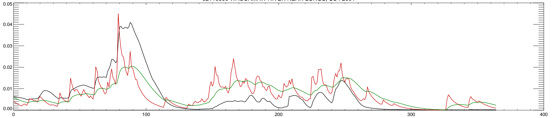
02110500 WACCAMAW RIVER NEAR LONGS, SC : 2002
