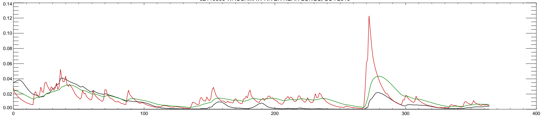
02110500 WACCAMAW RIVER NEAR LONGS, SC : 2011
