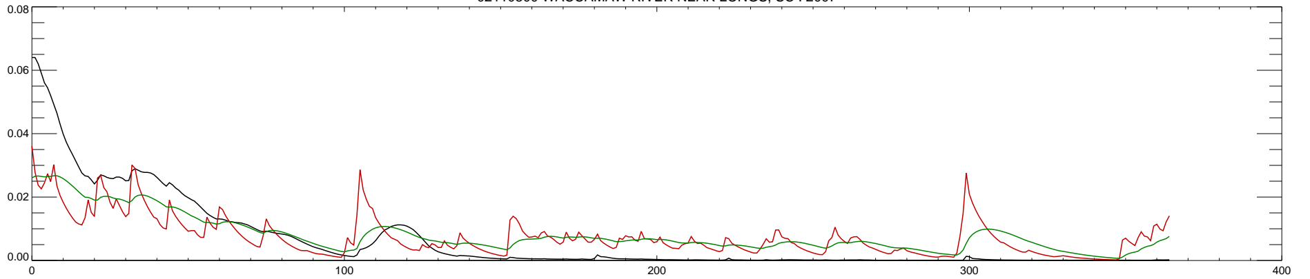
02110500 WACCAMAW RIVER NEAR LONGS, SC : 2008
