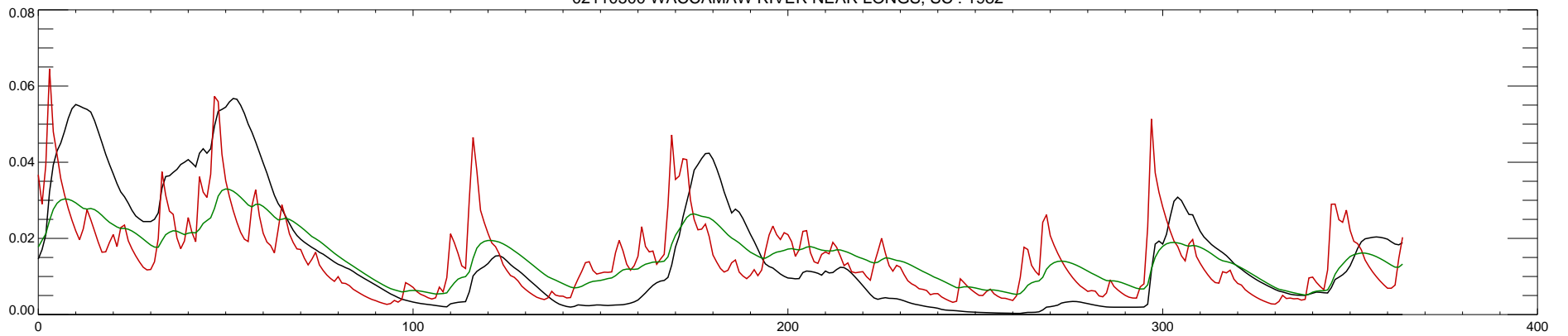
02110500 WACCAMAW RIVER NEAR LONGS, SC : 1982
