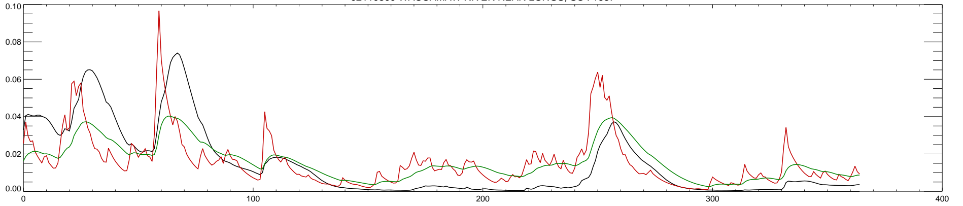
02110500 WACCAMAW RIVER NEAR LONGS, SC : 1988
