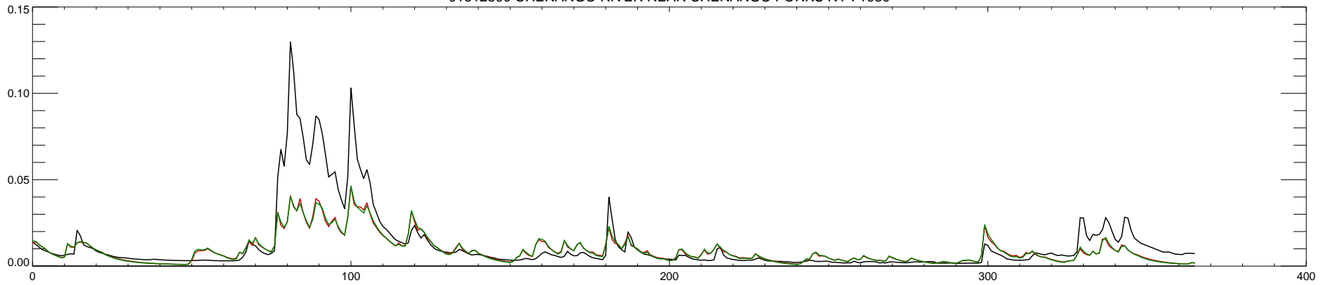
01512500 CHENANGO RIVER NEAR CHENANGO FORKS NY : 1981
