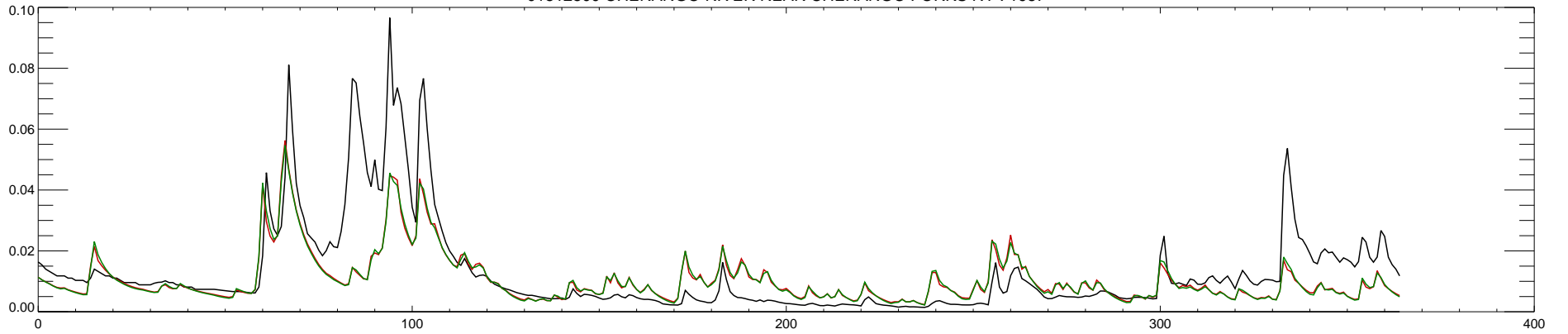
01512500 CHENANGO RIVER NEAR CHENANGO FORKS NY : 1988
