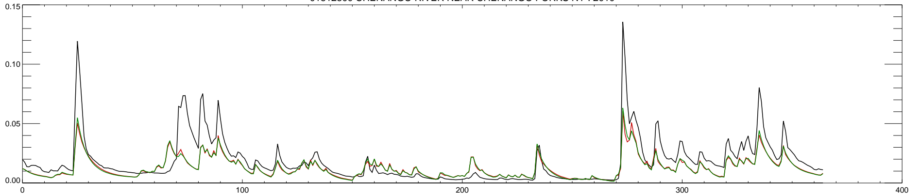
01512500 CHENANGO RIVER NEAR CHENANGO FORKS NY : 2011
