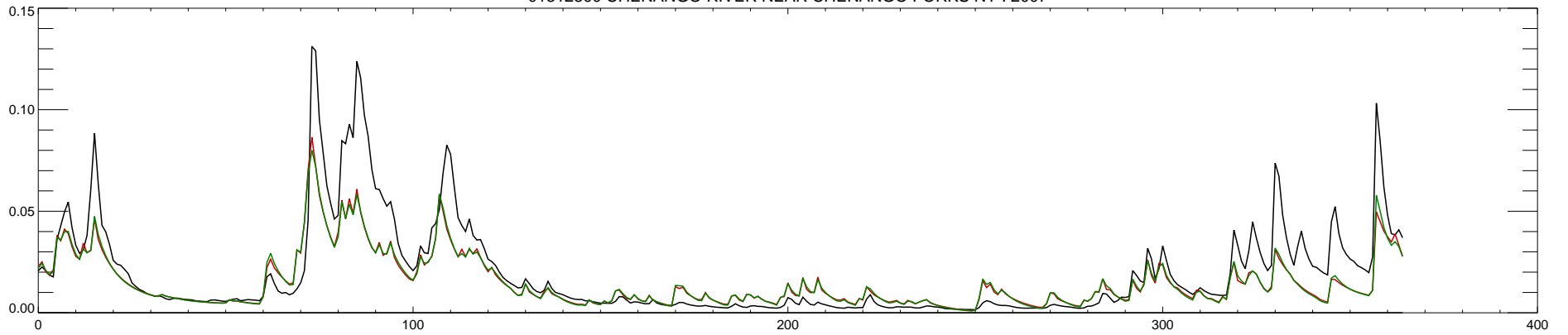
01512500 CHENANGO RIVER NEAR CHENANGO FORKS NY : 2008
