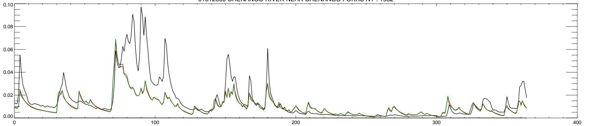
01512500 CHENANGO RIVER NEAR CHENANGO FORKS NY : 1982
