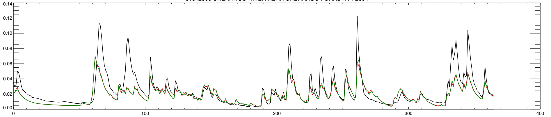
01512500 CHENANGO RIVER NEAR CHENANGO FORKS NY : 2005
