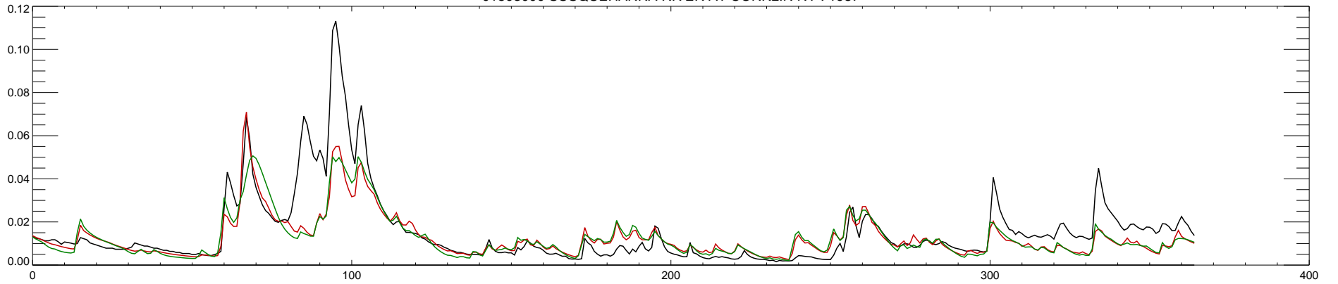
01503000 SUSQUEHANNA RIVER AT CONKLIN NY : 1988
