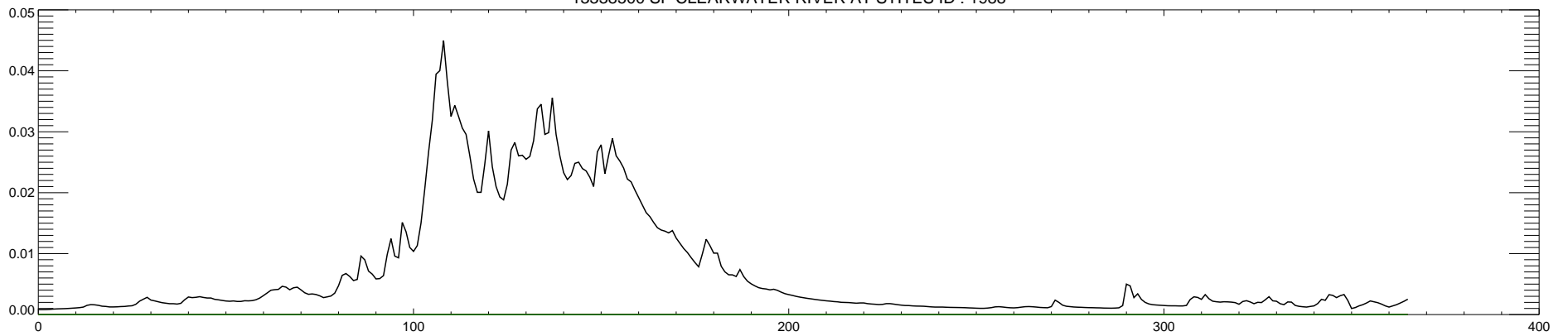
13338500 SF CLEARWATER RIVER AT STITES ID : 1988
