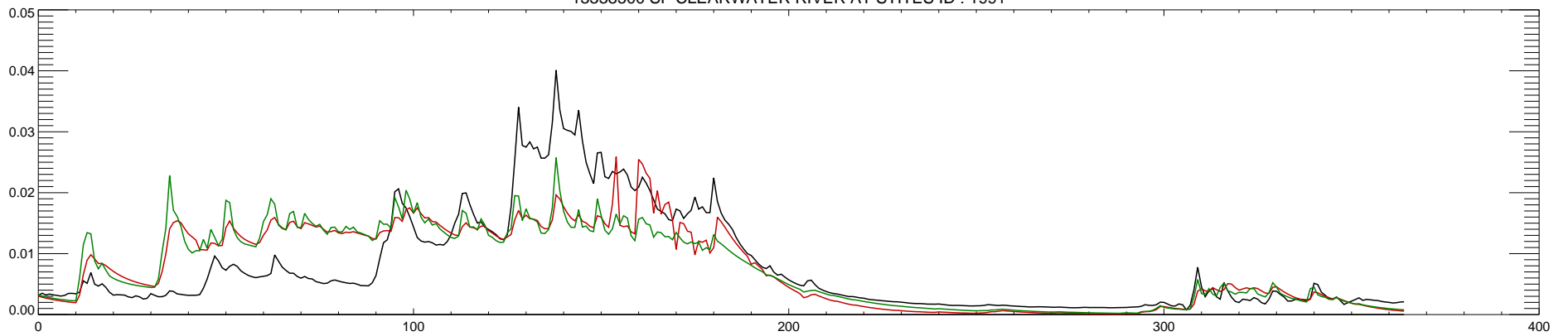
13338500 SF CLEARWATER RIVER AT STITES ID : 1991
