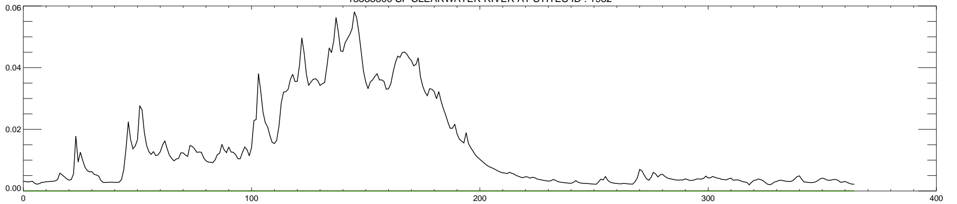
13338500 SF CLEARWATER RIVER AT STITES ID : 1982
