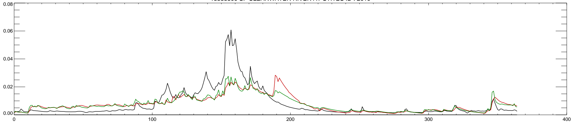
13338500 SF CLEARWATER RIVER AT STITES ID : 2011
