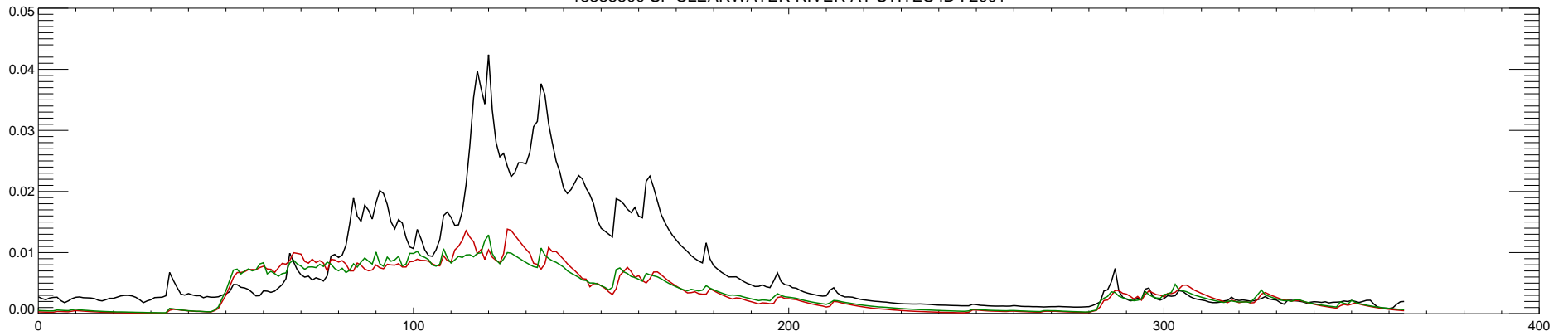
13338500 SF CLEARWATER RIVER AT STITES ID : 2002
