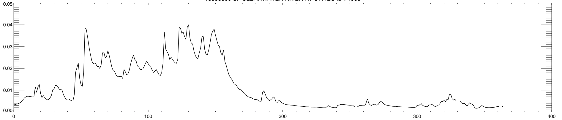
13338500 SF CLEARWATER RIVER AT STITES ID : 1987
