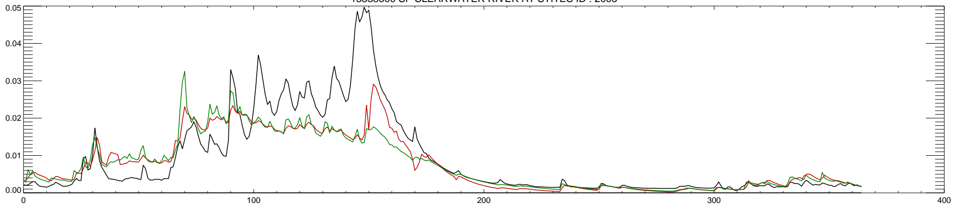
13338500 SF CLEARWATER RIVER AT STITES ID : 2003
