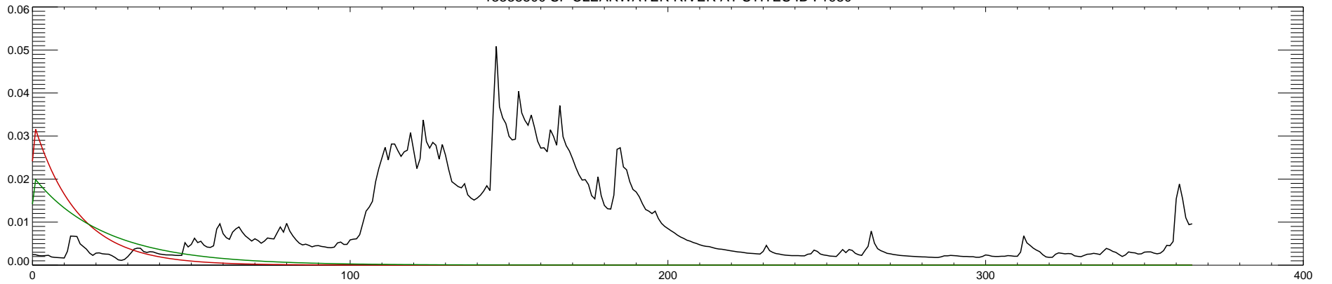
13338500 SF CLEARWATER RIVER AT STITES ID : 1981
