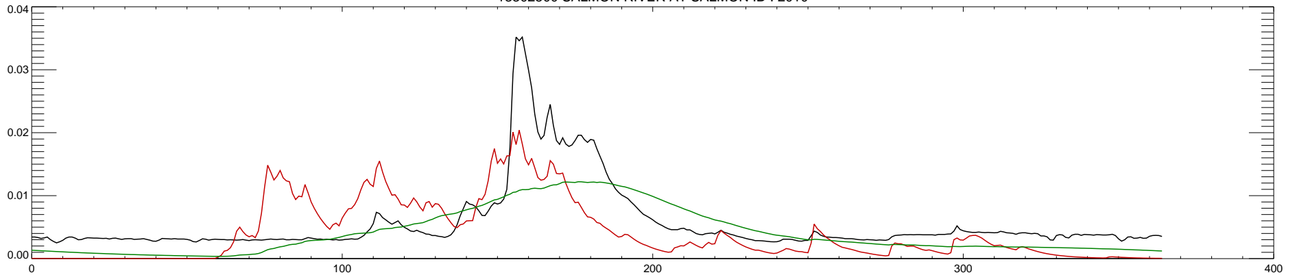
13302500 SALMON RIVER AT SALMON ID : 2011
