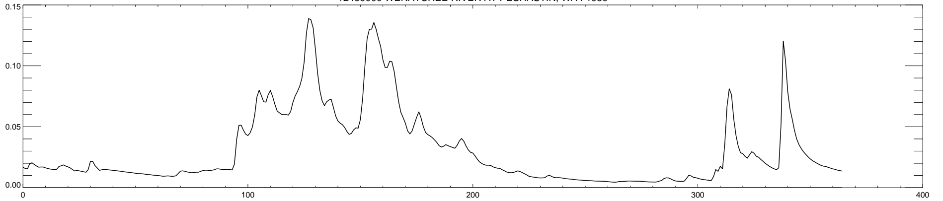
12459000 WENATCHEE RIVER AT PESHASTIN, WA : 1990
