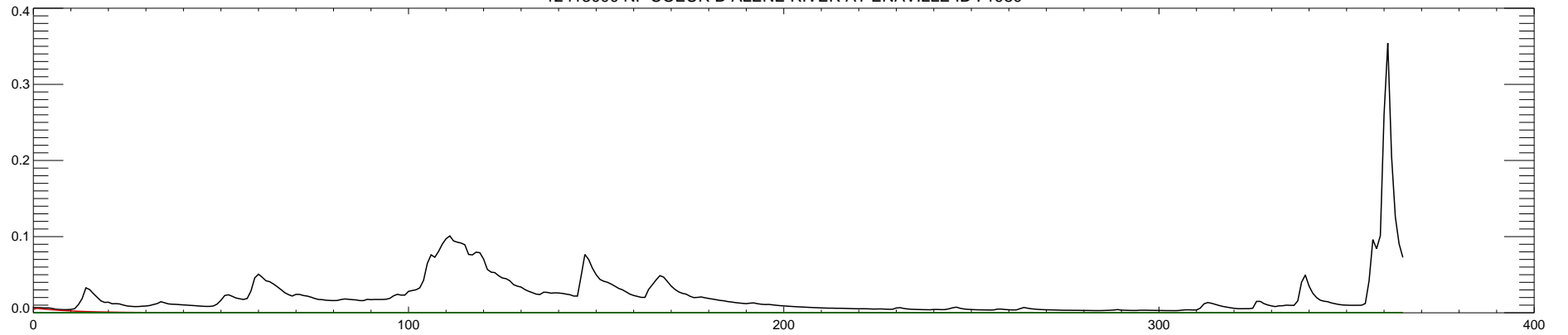
12413000 NF COEUR D ALENE RIVER AT ENAVILLE ID : 1981
