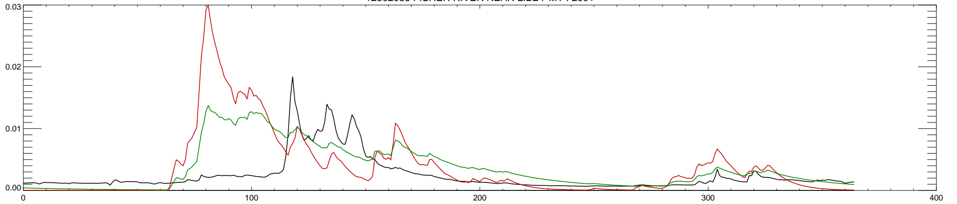
12302055 FISHER RIVER NEAR LIBBY MT : 2002
