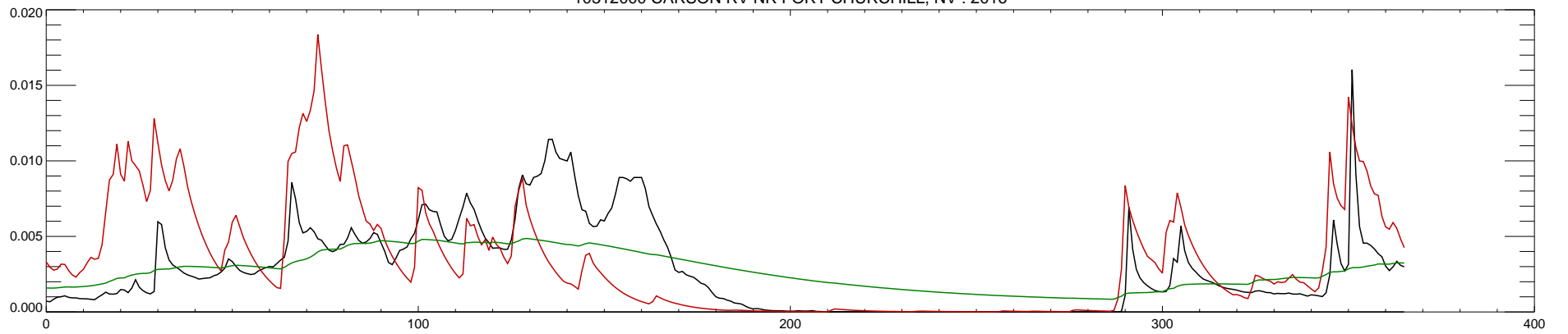
10312000 CARSON RV NR FORT CHURCHILL, NV : 2016
