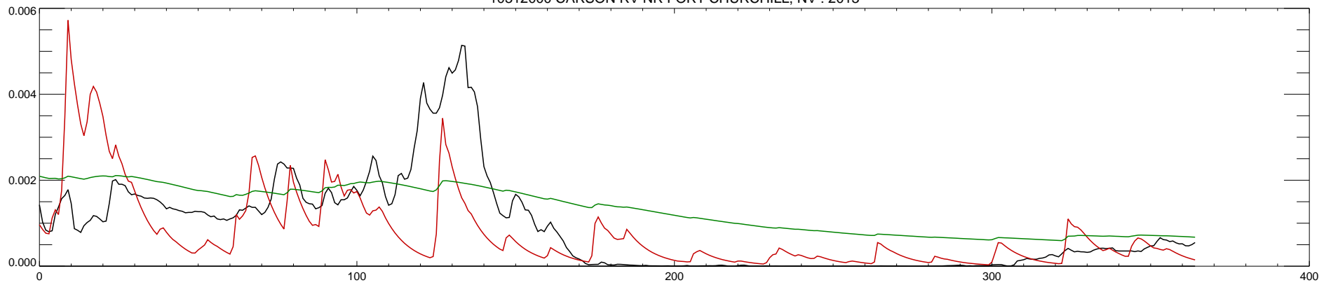
10312000 CARSON RV NR FORT CHURCHILL, NV : 2014
