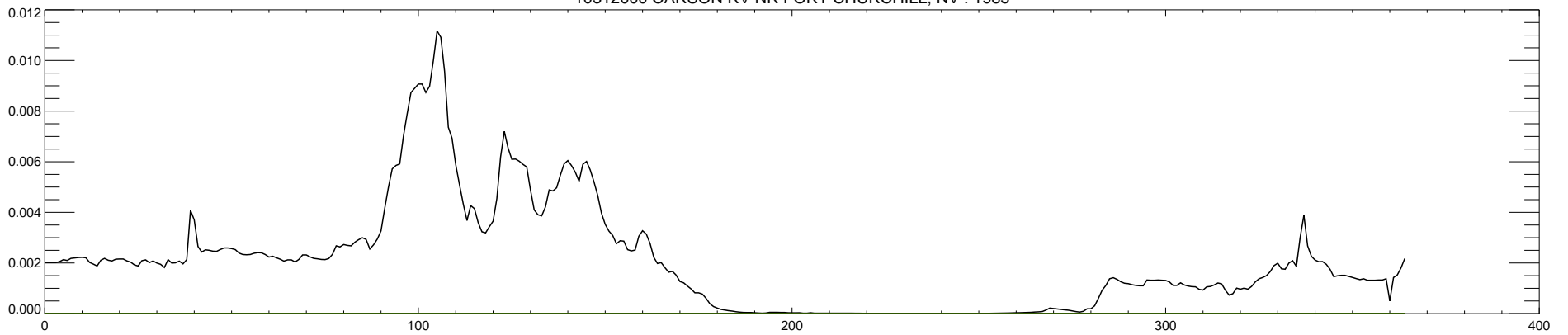
10312000 CARSON RV NR FORT CHURCHILL, NV : 1985
