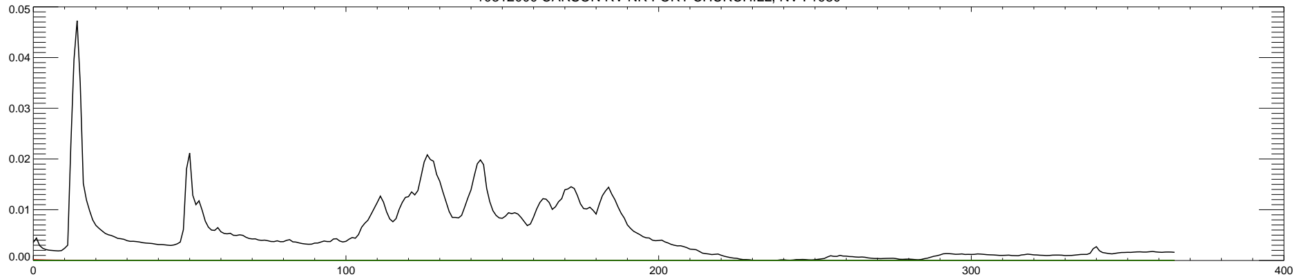
10312000 CARSON RV NR FORT CHURCHILL, NV : 1981
