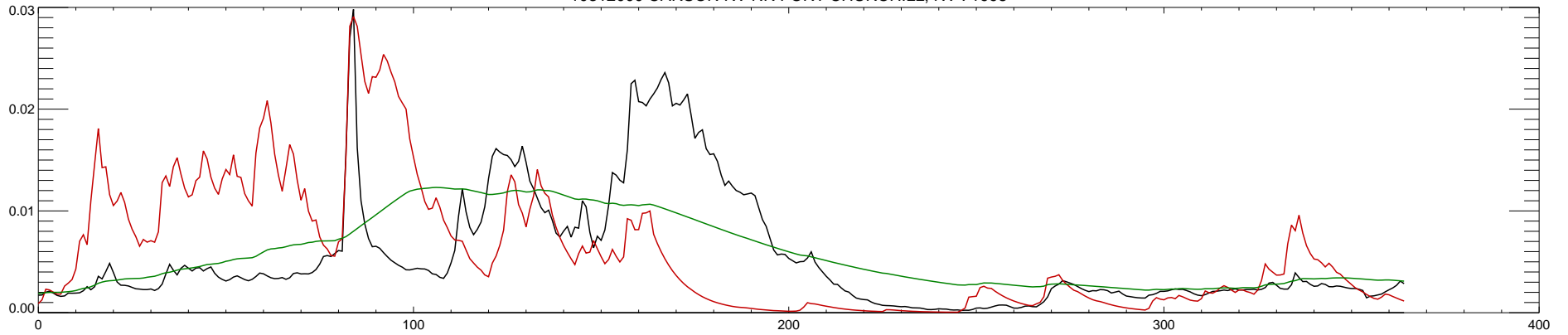
10312000 CARSON RV NR FORT CHURCHILL, NV : 1999
