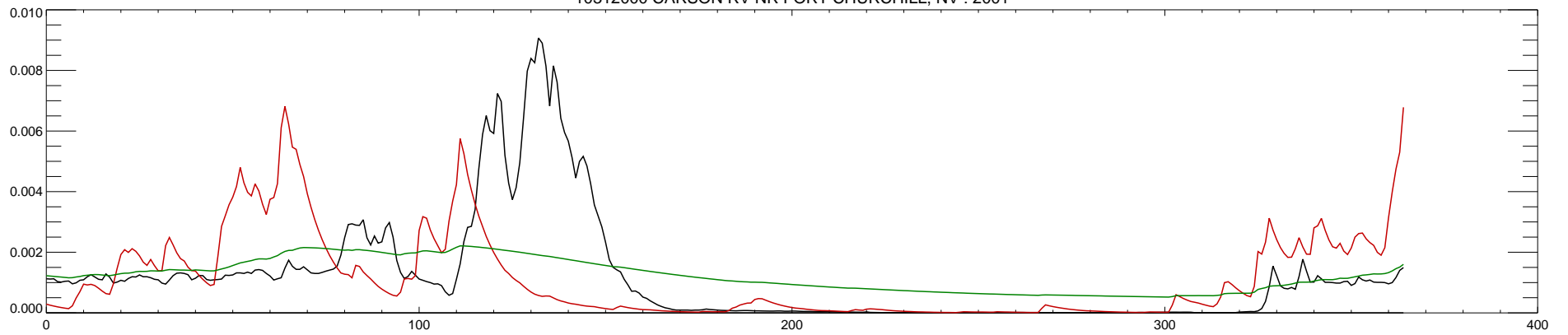
10312000 CARSON RV NR FORT CHURCHILL, NV : 2002
