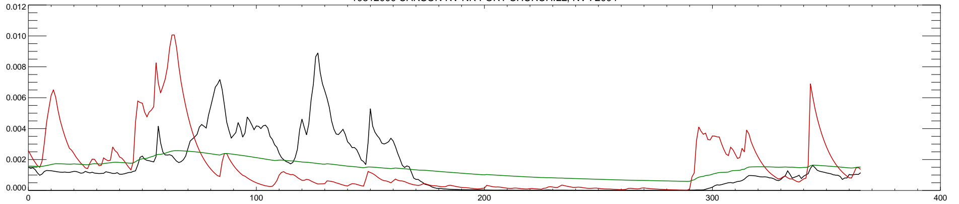
10312000 CARSON RV NR FORT CHURCHILL, NV : 2005
