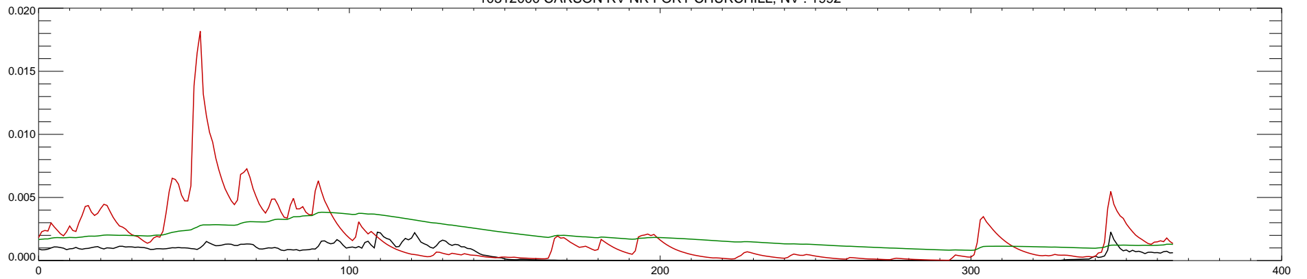
10312000 CARSON RV NR FORT CHURCHILL, NV : 1993
