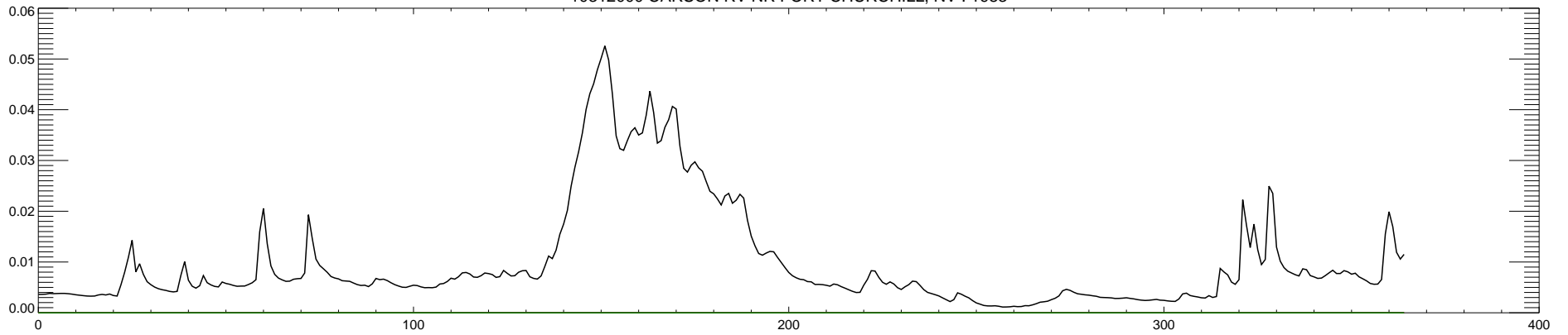
10312000 CARSON RV NR FORT CHURCHILL, NV : 1984
