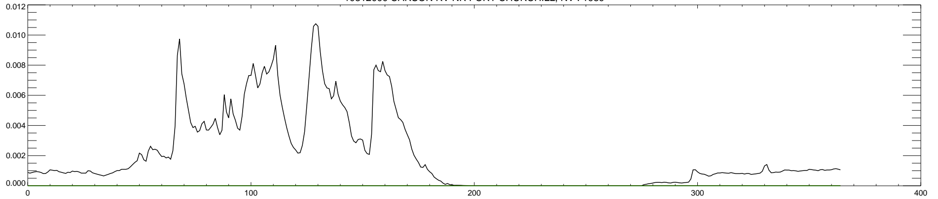
10312000 CARSON RV NR FORT CHURCHILL, NV : 1990
