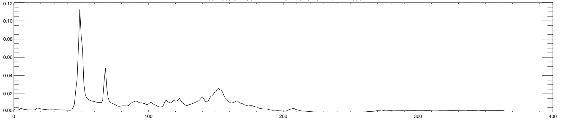
10312000 CARSON RV NR FORT CHURCHILL, NV : 1987
