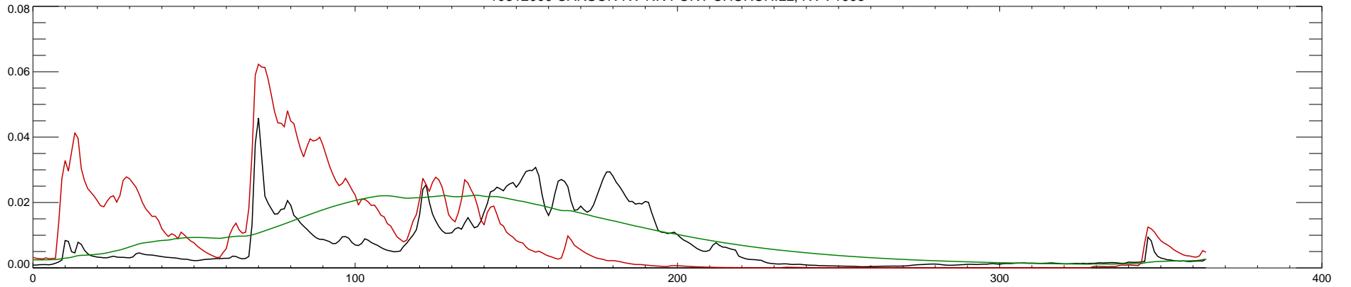
10312000 CARSON RV NR FORT CHURCHILL, NV : 1996
