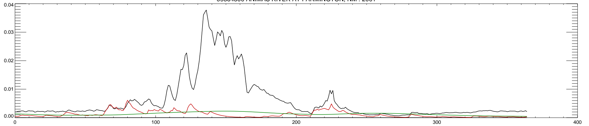
09364500 ANIMAS RIVER AT FARMINGTON, NM : 2002
