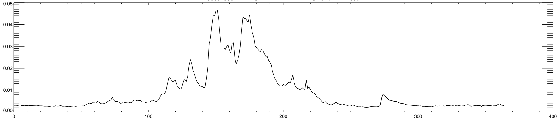
09364500 ANIMAS RIVER AT FARMINGTON, NM : 1984
