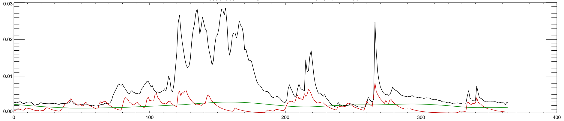
09364500 ANIMAS RIVER AT FARMINGTON, NM : 2008
